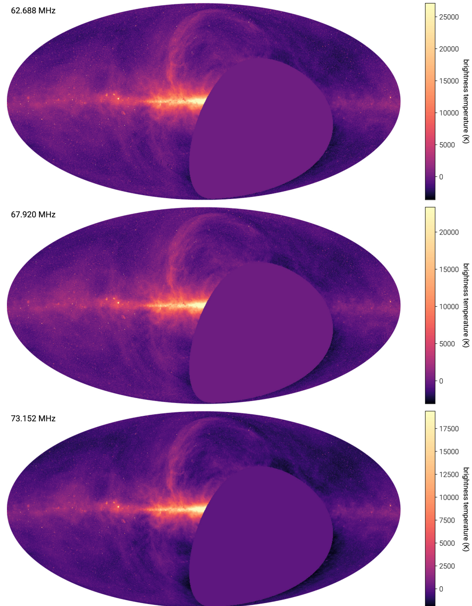
Figure 8. from The Radio Sky at Meter Wavelengths: m-mode Analysis Imaging with the OVRO-LWA null 2018 AJ 156 32 doi:10.3847/1538-3881/aac721 https://dx.doi.org/10.3847/1538-3881/aac721 © 2018. The American Astronomical Society. All rights reserved.
