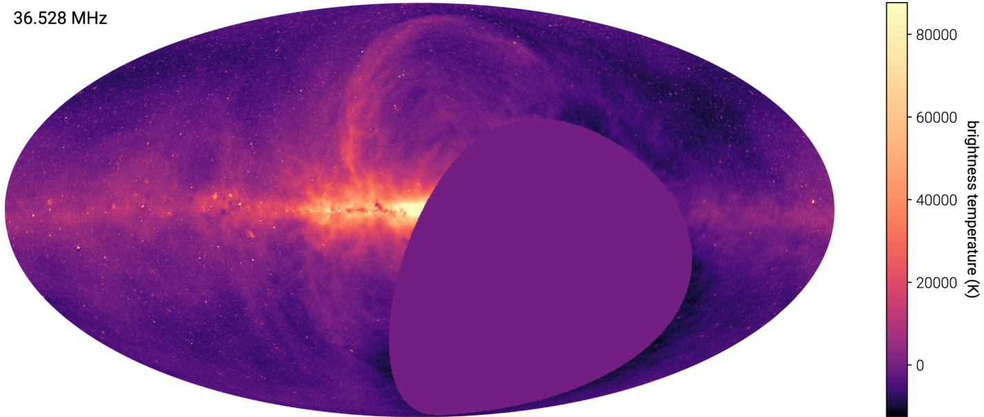
Figure 8. from The Radio Sky at Meter Wavelengths: m-mode Analysis Imaging with the OVRO-LWA null 2018 AJ 156 32 doi:10.3847/1538-3881/aac721 https://dx.doi.org/10.3847/1538-3881/aac721 © 2018. The American Astronomical Society. All rights reserved.
