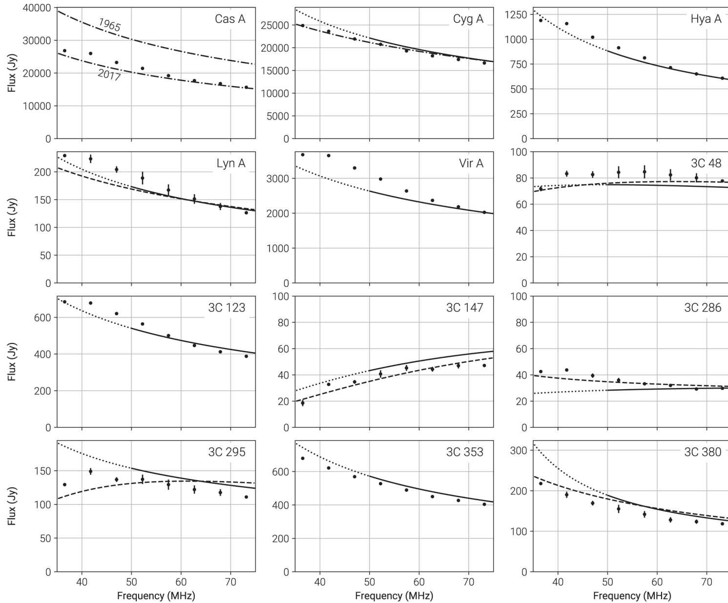
Figure 7. from The Radio Sky at Meter Wavelengths: m-mode Analysis Imaging with the OVRO-LWA null 2018 AJ 156 32 doi:10.3847/1538-3881/aac721 https://dx.doi.org/10.3847/1538-3881/aac721
