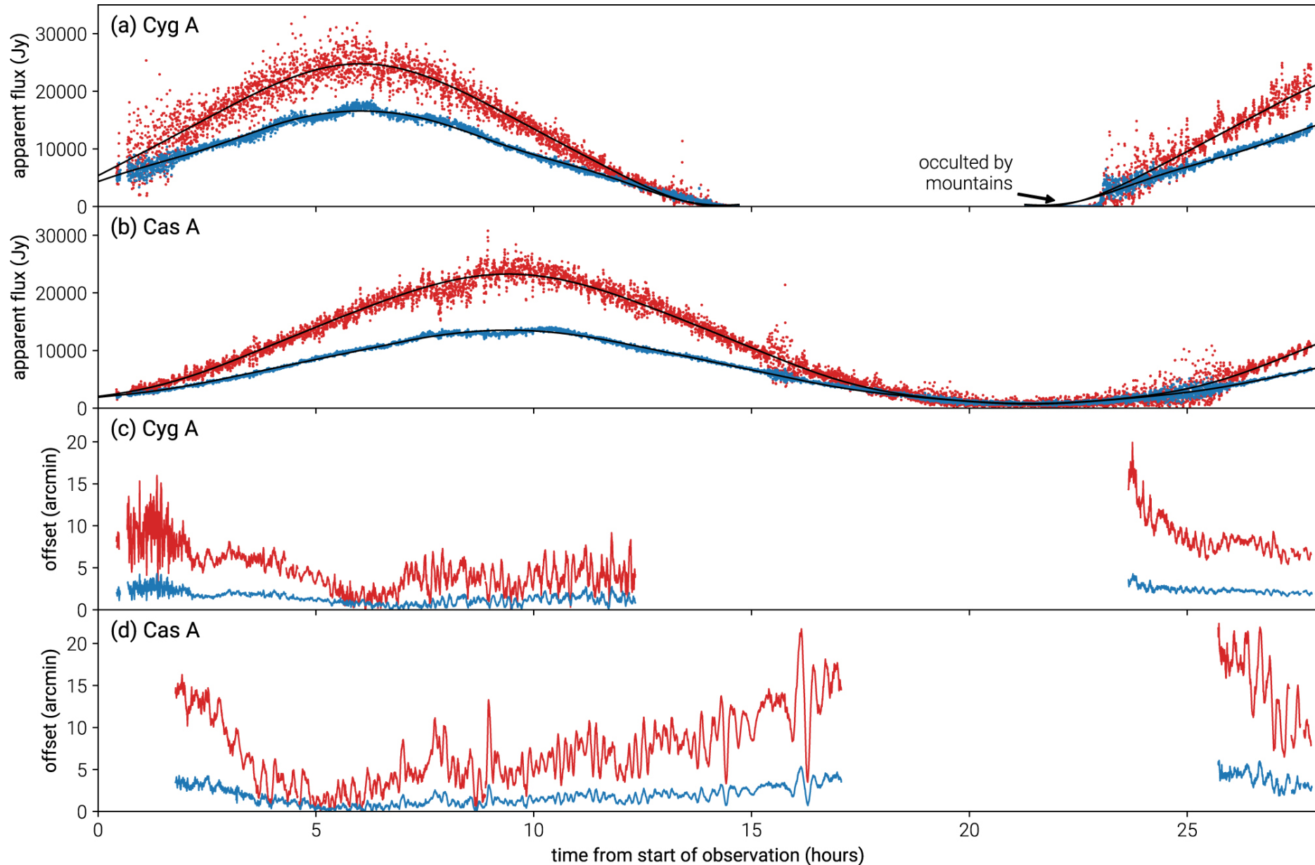
Figure 5. from The Radio Sky at Meter Wavelengths: m-mode Analysis Imaging with the OVRO-LWA null 2018 AJ 156 32 doi:10.3847/1538-3881/aac721 https://dx.doi.org/10.3847/1538-3881/aac721 © 2018. The American Astronomical Society. All rights reserved.
