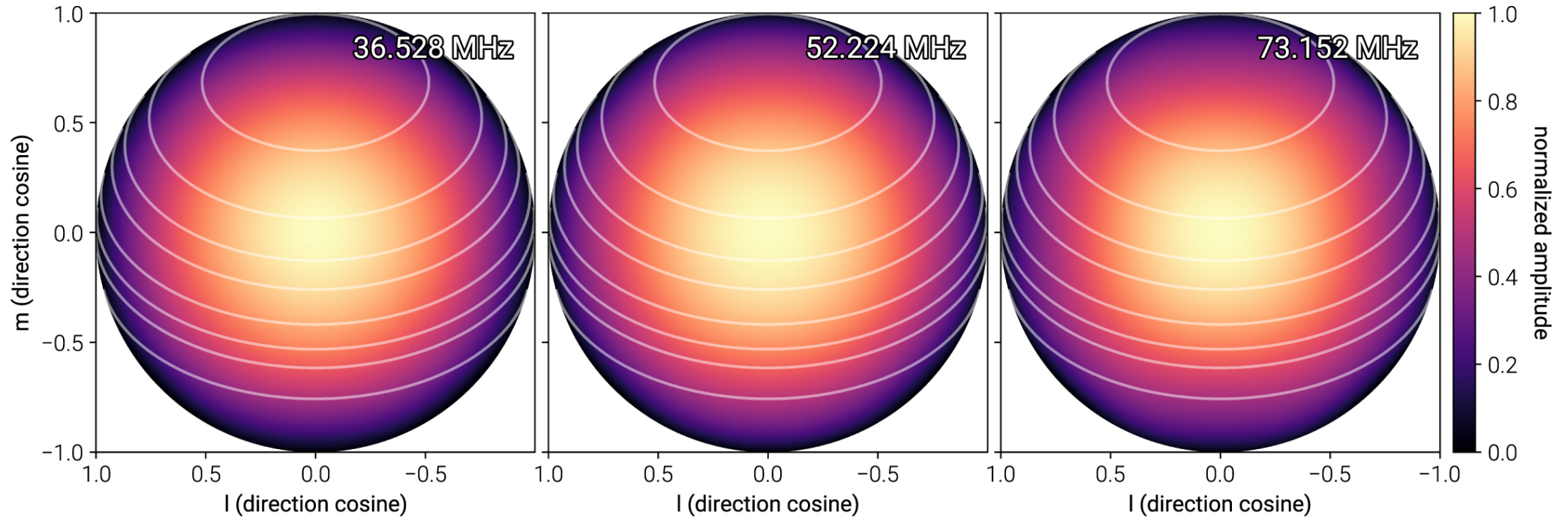
Figure 4. from The Radio Sky at Meter Wavelengths: m-mode Analysis Imaging with the OVRO-LWA null 2018 AJ 156 32 doi:10.3847/1538-3881/aac721 https://dx.doi.org/10.3847/1538-3881/aac721 © 2018. The American Astronomical Society. All rights reserved.
