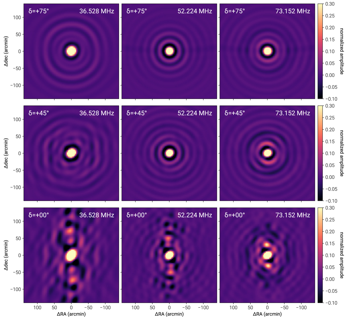
Figure 3. from The Radio Sky at Meter Wavelengths: m-mode Analysis Imaging with the OVRO-LWA null 2018 AJ 156 32 doi:10.3847/1538-3881/aac721 https://dx.doi.org/10.3847/1538-3881/aac721 © 2018. The American Astronomical Society. All rights reserved.
