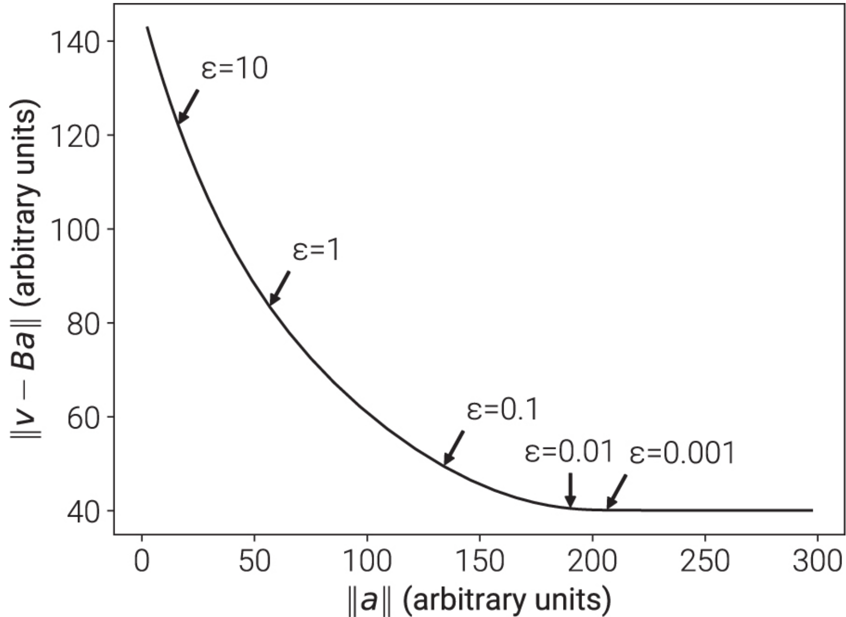
Figure 1. from The Radio Sky at Meter Wavelengths: m-mode Analysis Imaging with the OVRO-LWA null 2018 AJ 156 32 doi:10.3847/1538-3881/aac721 https://dx.doi.org/10.3847/1538-3881/aac721 © 2018. The American Astronomical Society. All rights reserved.
