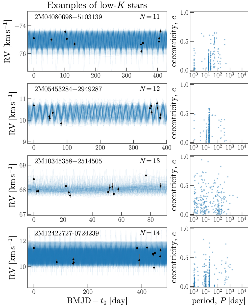
Figure 8. from Binary Companions of Evolved Stars in APOGEE DR14: Search Method and Catalog of 5000 Companions null 2018 AJ 156 18 doi:10.3847/1538-3881/aac387 https://dx.doi.org/10.3847/1538-3881/aac387
