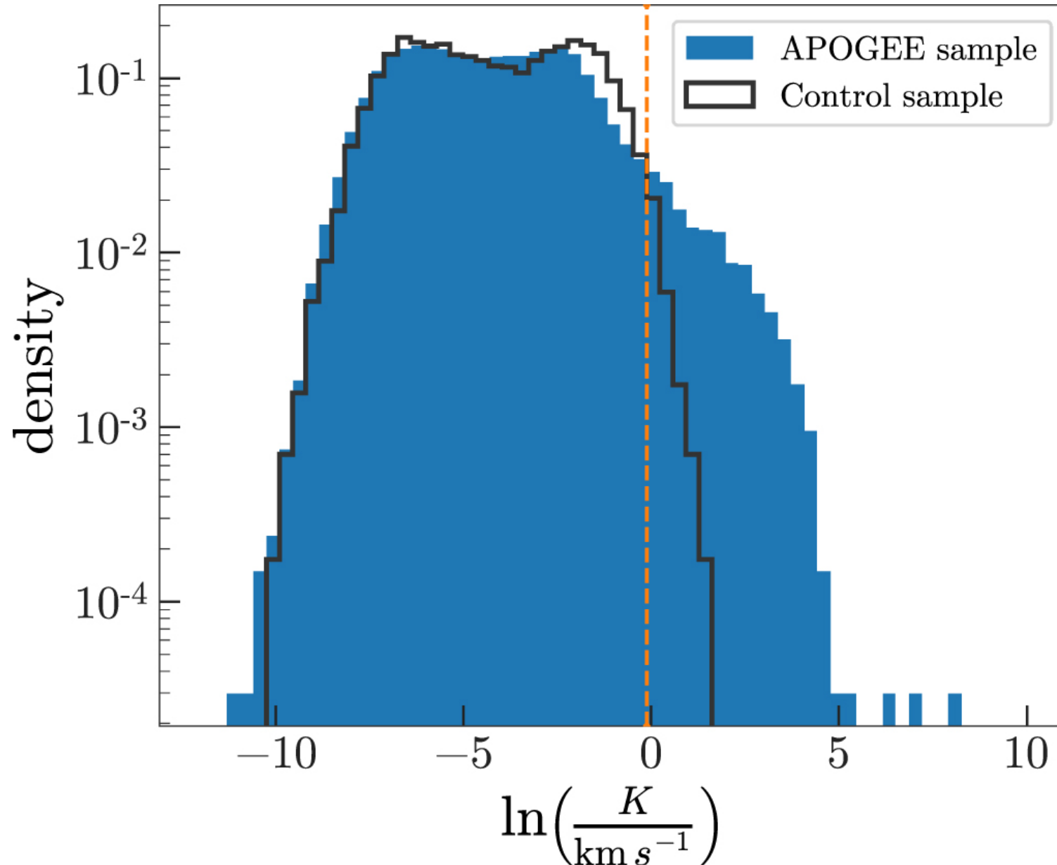
Figure 4. from Binary Companions of Evolved Stars in APOGEE DR14: Search Method and Catalog of 5000 Companions null 2018 AJ 156 18 doi:10.3847/1538-3881/aac387 https://dx.doi.org/10.3847/1538-3881/aac387 © 2018. The American Astronomical Society. All rights reserved.
