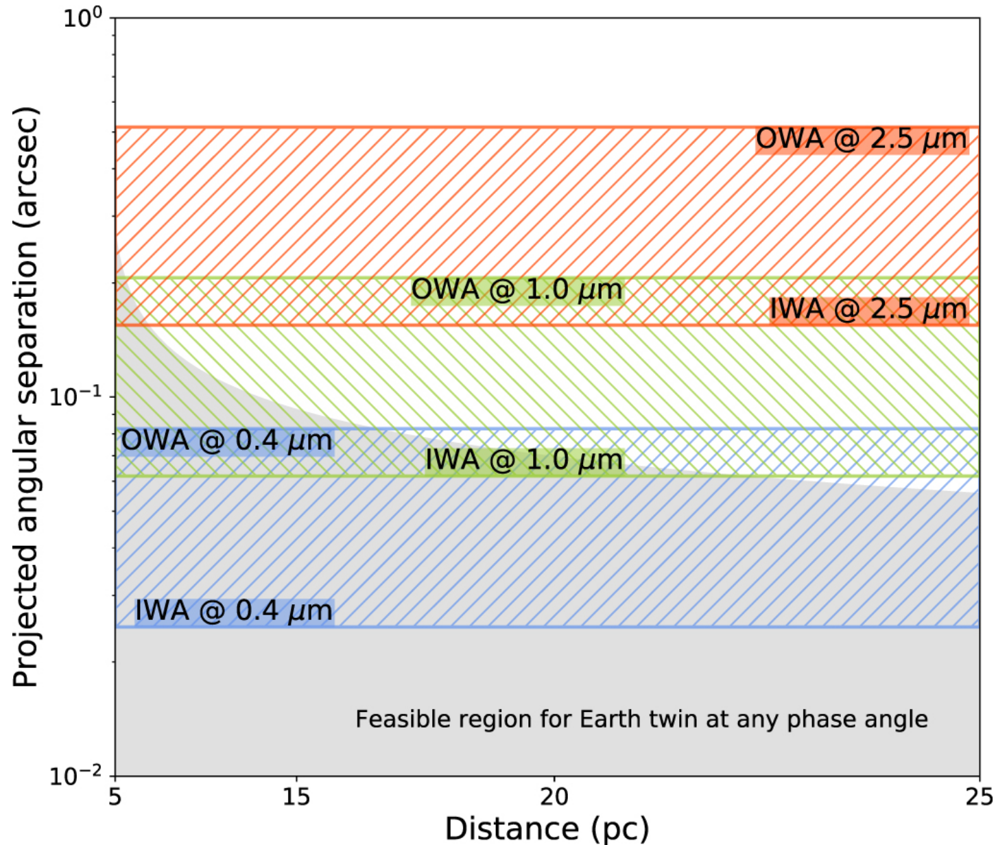
Figure 6. from The Direct Imaging Search for Earth 2.0: Quantifying Biases and Planetary False Positives null 2018 AJ 155 230 doi:10.3847/1538-3881/aabb02 https://dx.doi.org/10.3847/1538-3881/aabb02 © 2018. The American Astronomical Society. All rights reserved.
