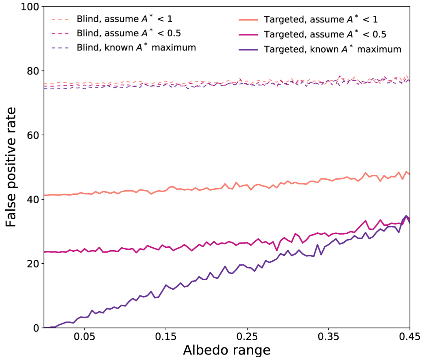
Figure 5. from The Direct Imaging Search for Earth 2.0: Quantifying Biases and Planetary False Positives null 2018 AJ 155 230 doi:10.3847/1538-3881/aabb02 https://dx.doi.org/10.3847/1538-3881/aabb02
