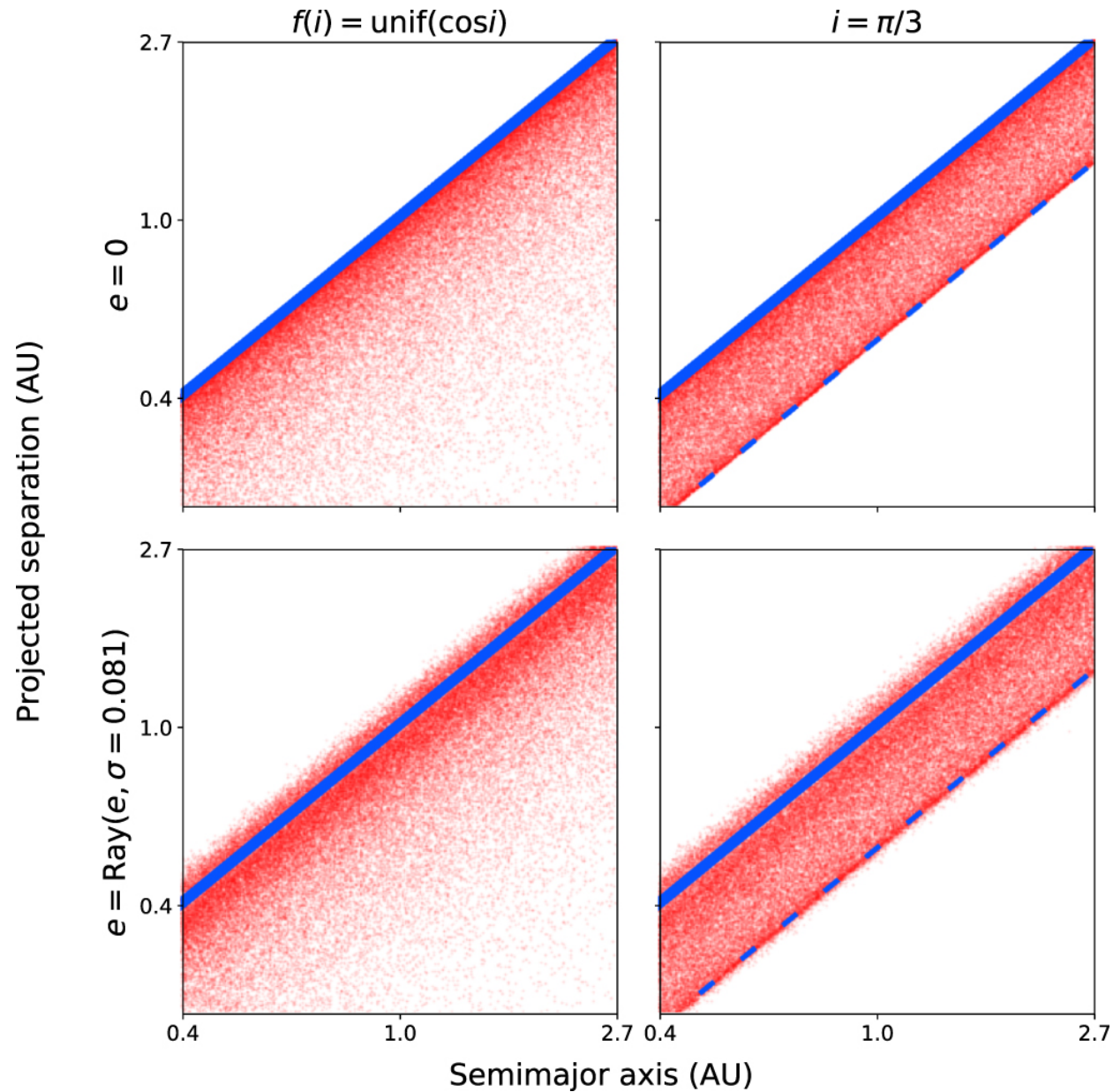
Figure 4. from The Direct Imaging Search for Earth 2.0: Quantifying Biases and Planetary False Positives null 2018 AJ 155 230 doi:10.3847/1538-3881/aabb02 https://dx.doi.org/10.3847/1538-3881/aabb02 © 2018. The American Astronomical Society. All rights reserved.
