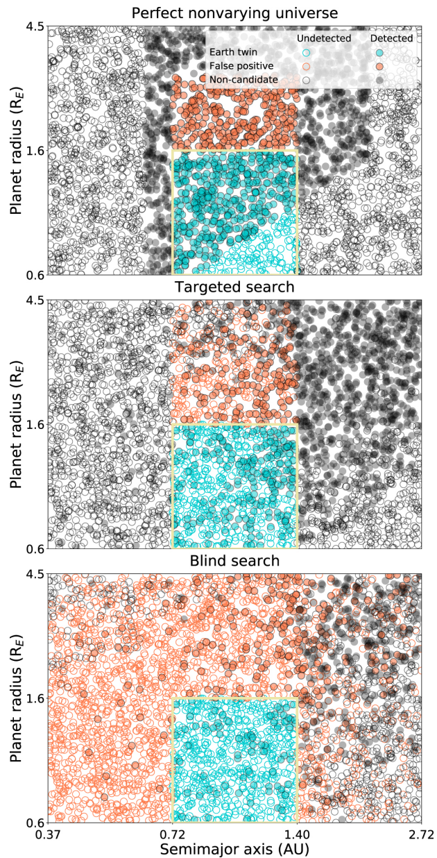
Figure 1. from The Direct Imaging Search for Earth 2.0: Quantifying Biases and Planetary False Positives null 2018 AJ 155 230 doi:10.3847/1538-3881/aabb02 https://dx.doi.org/10.3847/1538-3881/aabb02 © 2018. The American Astronomical Society. All rights reserved.
