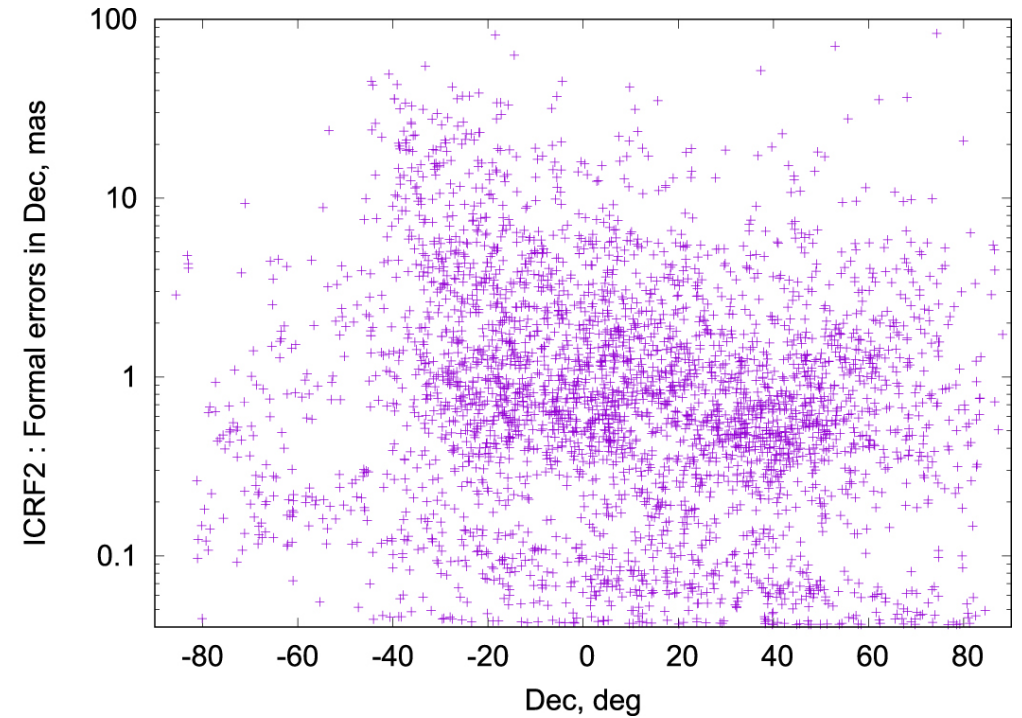
Figure 7. from Toward the ICRF3: Astrometric Comparison of the USNO 2016A VLBI Solution with ICRF2 and Gaia DR1 null 2018 AJ 155 229 doi:10.3847/1538-3881/aabafa https://dx.doi.org/10.3847/1538-3881/aabafa
