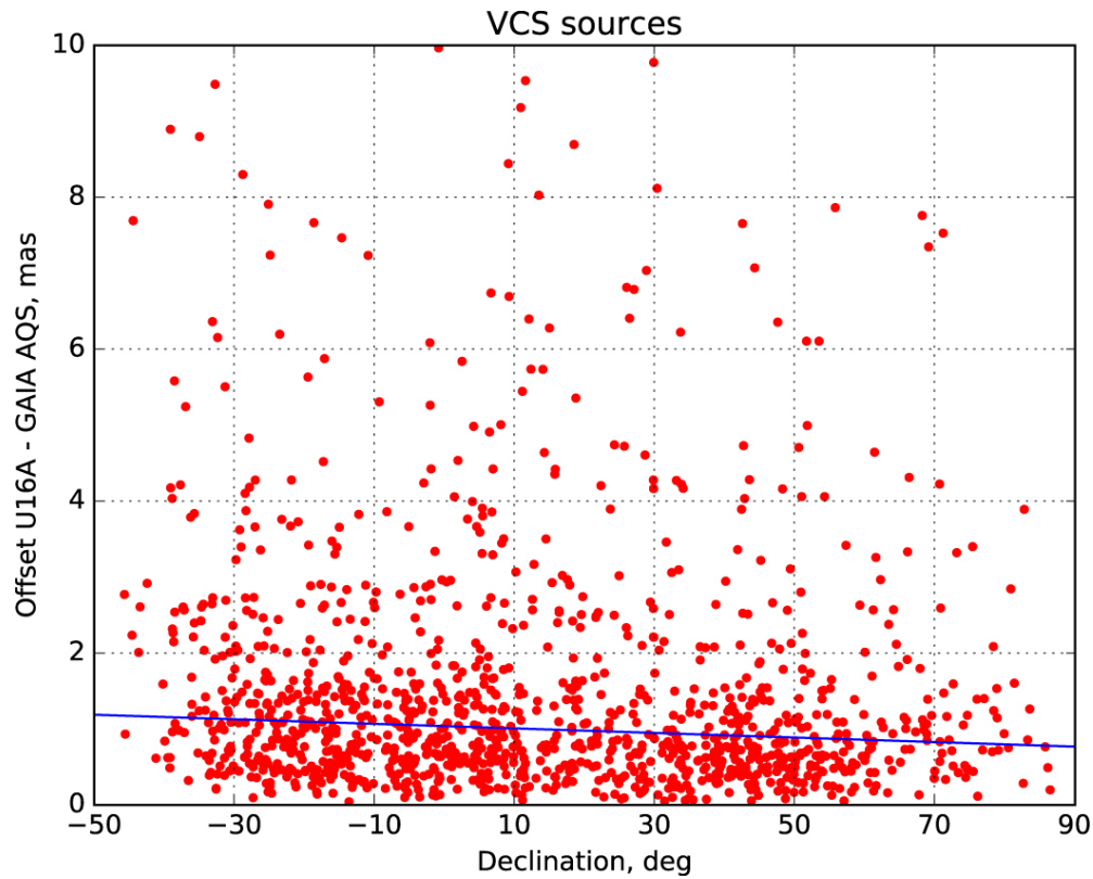
Figure 5. from Toward the ICRF3: Astrometric Comparison of the USNO 2016A VLBI Solution with ICRF2 and Gaia DR1 null 2018 AJ 155 229 doi:10.3847/1538-3881/aabafa https://dx.doi.org/10.3847/1538-3881/aabafa © 2018. The American Astronomical Society. All rights reserved.
