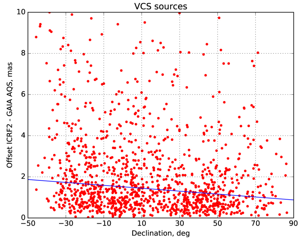
Figure 5. from Toward the ICRF3: Astrometric Comparison of the USNO 2016A VLBI Solution with ICRF2 and Gaia DR1 null 2018 AJ 155 229 doi:10.3847/1538-3881/aabafa https://dx.doi.org/10.3847/1538-3881/aabafa © 2018. The American Astronomical Society. All rights reserved.
