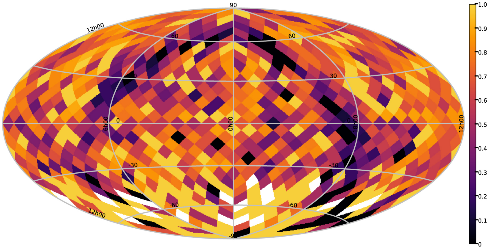
Figure 4. from Toward the ICRF3: Astrometric Comparison of the USNO 2016A VLBI Solution with ICRF2 and Gaia DR1 null 2018 AJ 155 229 doi:10.3847/1538-3881/aabafa https://dx.doi.org/10.3847/1538-3881/aabafa © 2018. The American Astronomical Society. All rights reserved.
