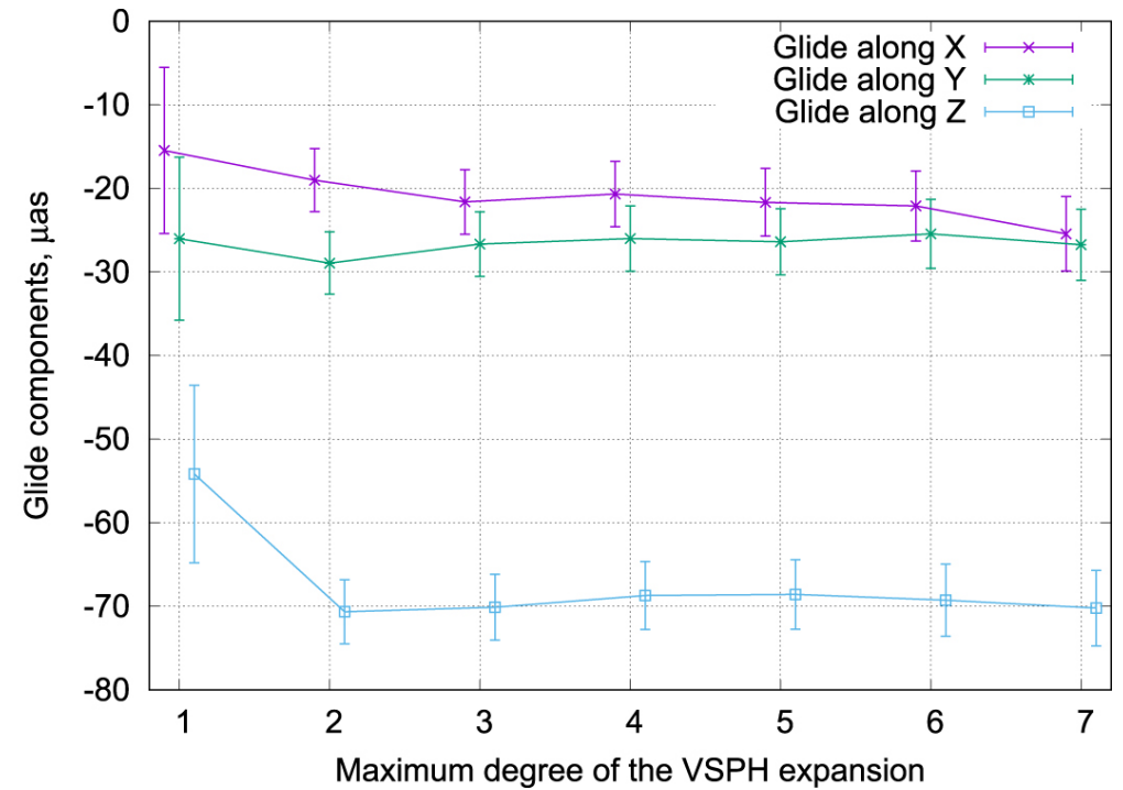
Figure 3. from Toward the ICRF3: Astrometric Comparison of the USNO 2016A VLBI Solution with ICRF2 and Gaia DR1 null 2018 AJ 155 229 doi:10.3847/1538-3881/aabafa https://dx.doi.org/10.3847/1538-3881/aabafa © 2018. The American Astronomical Society. All rights reserved.
