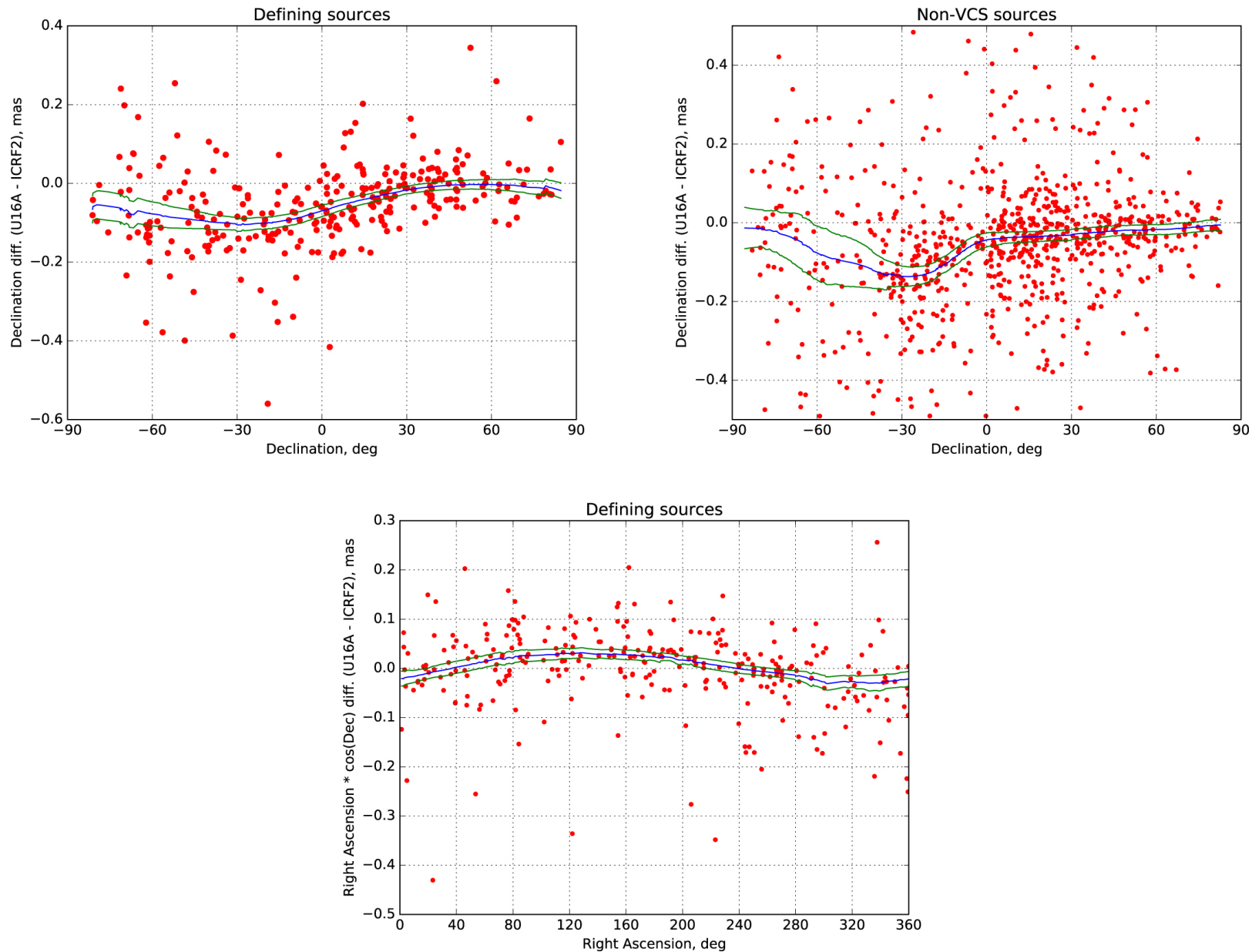
Figure 2. from Toward the ICRF3: Astrometric Comparison of the USNO 2016A VLBI Solution with ICRF2 and Gaia DR1 null 2018 AJ 155 229 doi:10.3847/1538-3881/aabafa https://dx.doi.org/10.3847/1538-3881/aabafa © 2018. The American Astronomical Society. All rights reserved.
