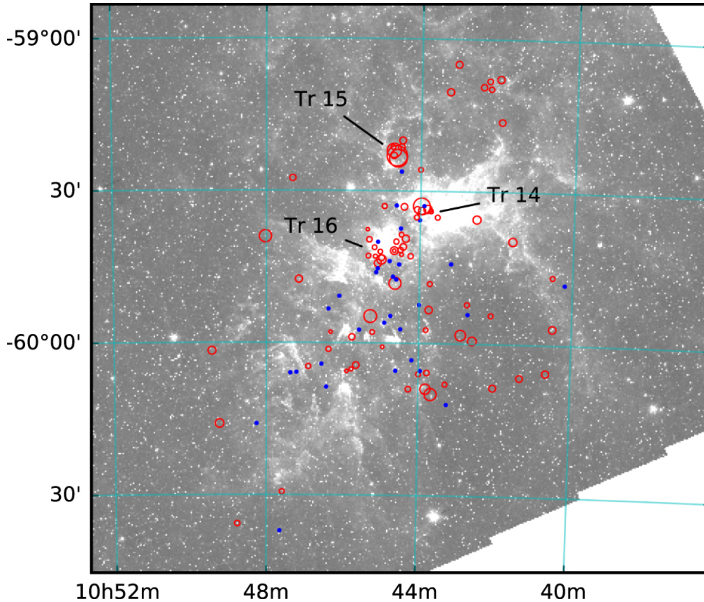
Figure 3. from Stellar Parameters and Radial Velocities of Hot Stars in the Carina Nebula null 2018 AJ 155 190 doi:10.3847/1538-3881/aab70d https://dx.doi.org/10.3847/1538-3881/aab70d © 2018. The American Astronomical Society. All rights reserved.
