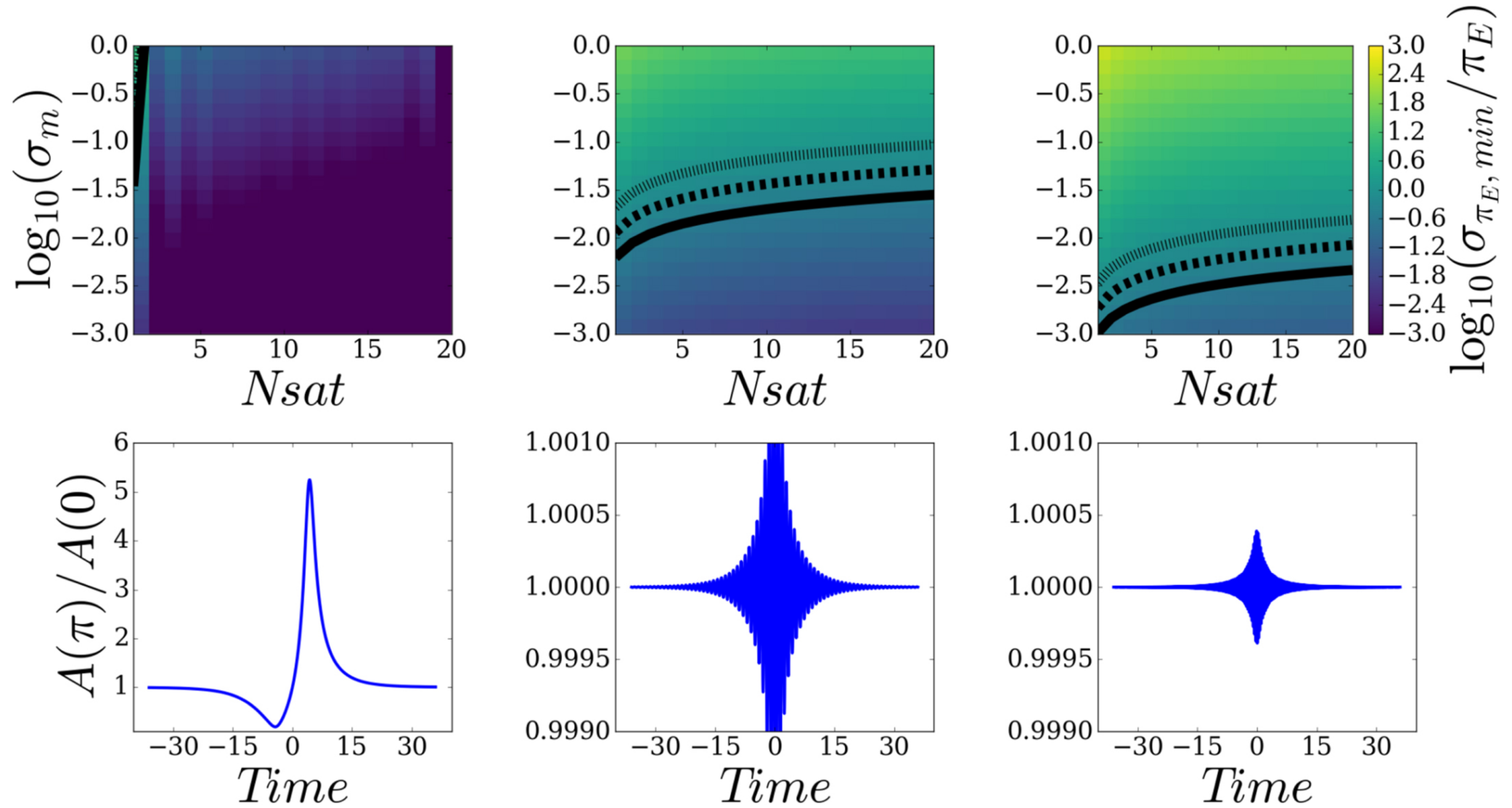
Figure 4. from Measuring the Microlensing Parallax from Various Space Observatories null 2018 AJ 155 191 doi:10.3847/1538-3881/aab3c8 https://dx.doi.org/10.3847/1538-3881/aab3c8 © 2018. The American Astronomical Society. All rights reserved.
