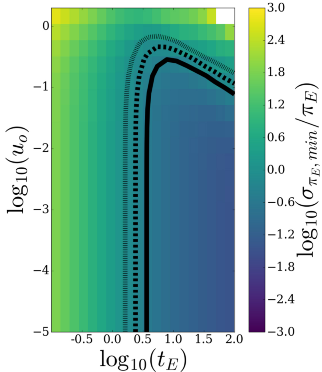
Figure 2. from Measuring the Microlensing Parallax from Various Space Observatories null 2018 AJ 155 191 doi:10.3847/1538-3881/aab3c8 https://dx.doi.org/10.3847/1538-3881/aab3c8 © 2018. The American Astronomical Society. All rights reserved.
