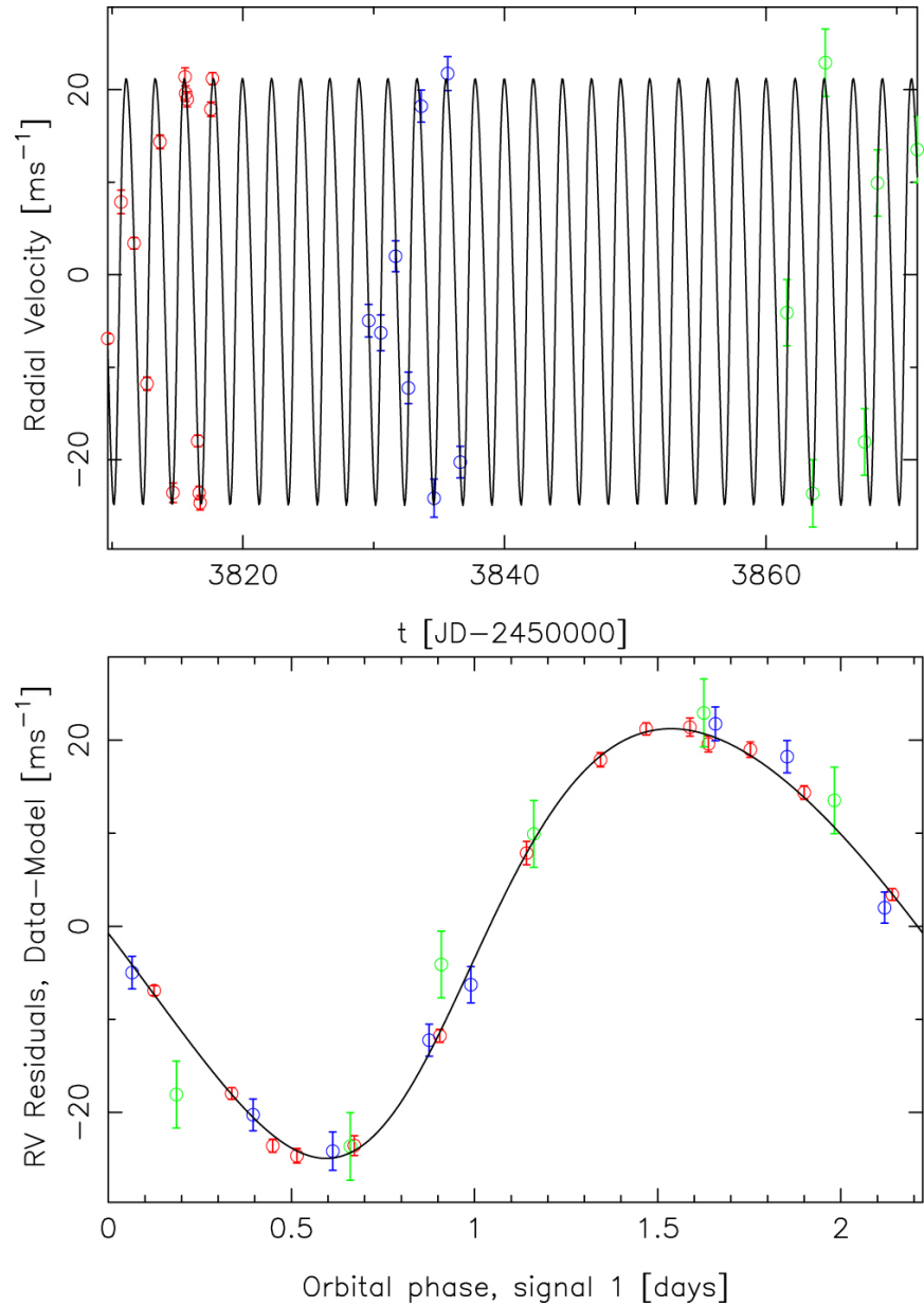
Figure 9. from AD Leonis: Radial Velocity Signal of Stellar Rotation or Spin–Orbit Resonance? null 2018 AJ 155 192 doi:10.3847/1538-3881/aab09c https://dx.doi.org/10.3847/1538-3881/aab09c © 2018. The American Astronomical Society.
