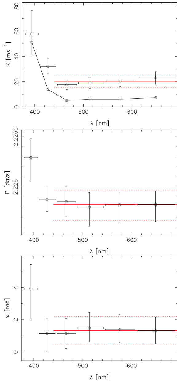
Figure 8. from AD Leonis: Radial Velocity Signal of Stellar Rotation or Spin–Orbit Resonance? null 2018 AJ 155 192 doi:10.3847/1538-3881/aab09c https://dx.doi.org/10.3847/1538-3881/aab09c © 2018. The American Astronomical Society.
