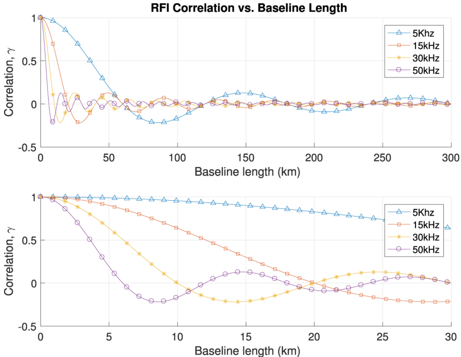
Figure 3. from Subarray Processing for Projection-based RFI Mitigation in Radio Astronomical Interferometers null 2018 AJ 155 146 doi:10.3847/1538-3881/aaae6f https://dx.doi.org/10.3847/1538-3881/aaae6f © 2018. The American Astronomical Society. All rights reserved.
