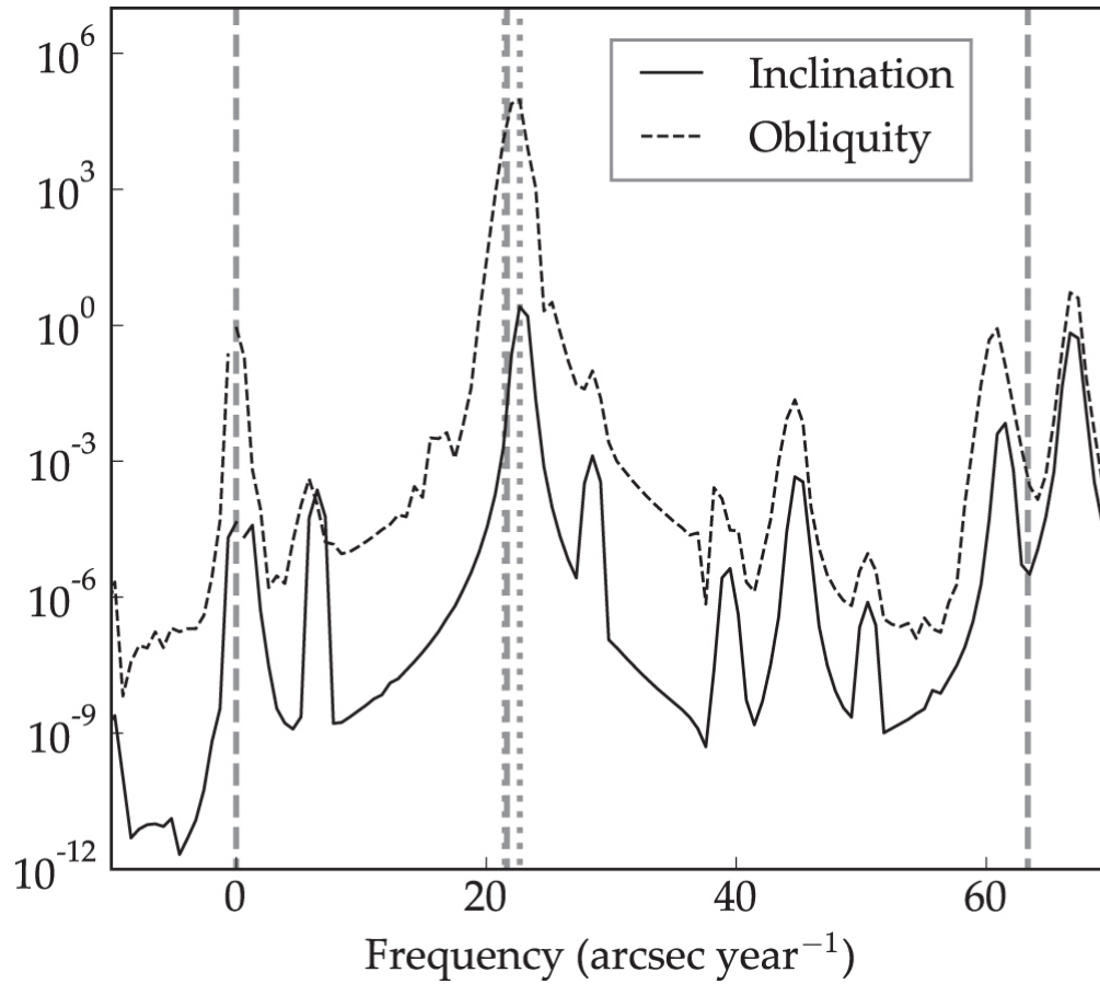
Figure 9. from Exo-Milankovitch Cycles. I. Orbits and Rotation States null 2018 AJ 155 60 doi:10.3847/1538-3881/aaa301 https://dx.doi.org/10.3847/1538-3881/aaa301 © 2018. The American Astronomical Society. All rights reserved.
