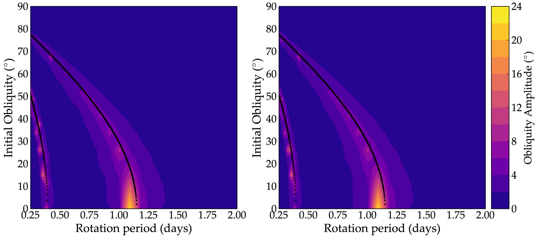
Figure 6. from Exo-Milankovitch Cycles. I. Orbits and Rotation States null 2018 AJ 155 60 doi:10.3847/1538-3881/aaa301 https://dx.doi.org/10.3847/1538-3881/aaa301 © 2018. The American Astronomical Society. All rights reserved.
