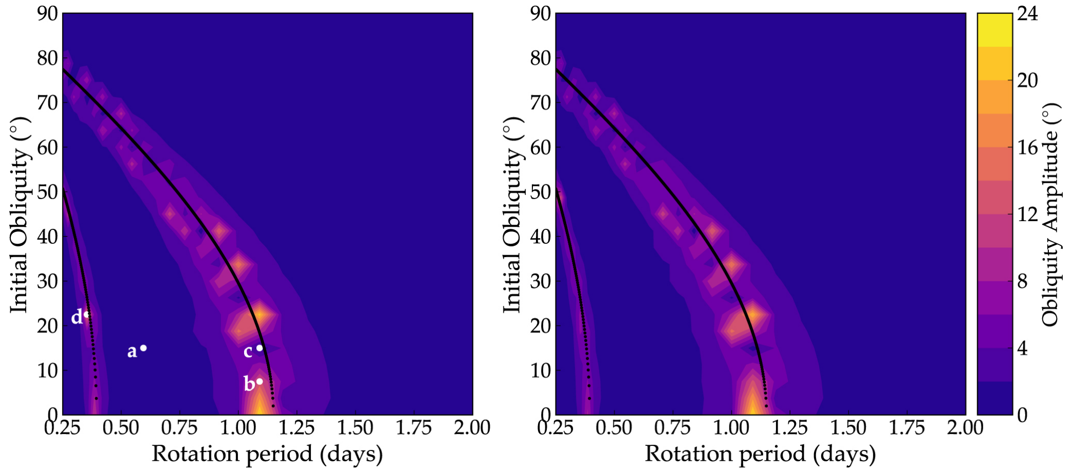
Figure 5. from Exo-Milankovitch Cycles. I. Orbits and Rotation States null 2018 AJ 155 60 doi:10.3847/1538-3881/aaa301 https://dx.doi.org/10.3847/1538-3881/aaa301 © 2018. The American Astronomical Society. All rights reserved.
