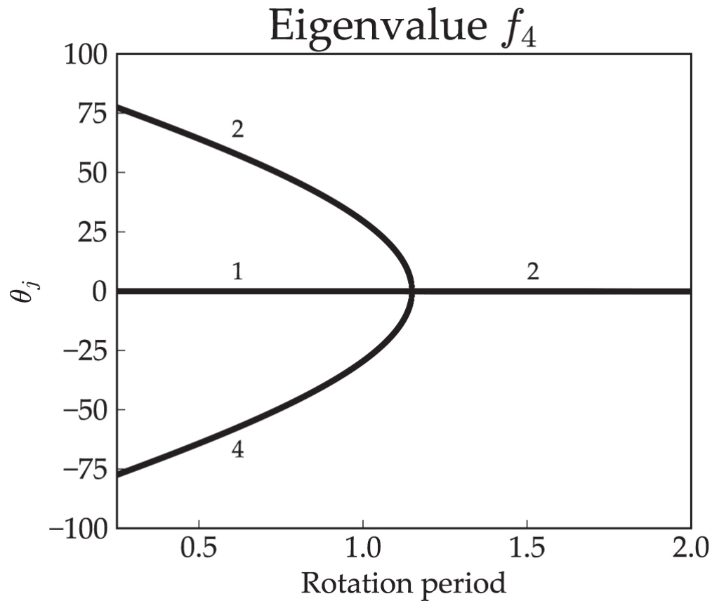
Figure 4. from Exo-Milankovitch Cycles. I. Orbits and Rotation States null 2018 AJ 155 60 doi:10.3847/1538-3881/aaa301 https://dx.doi.org/10.3847/1538-3881/aaa301 © 2018. The American Astronomical Society. All rights reserved.
