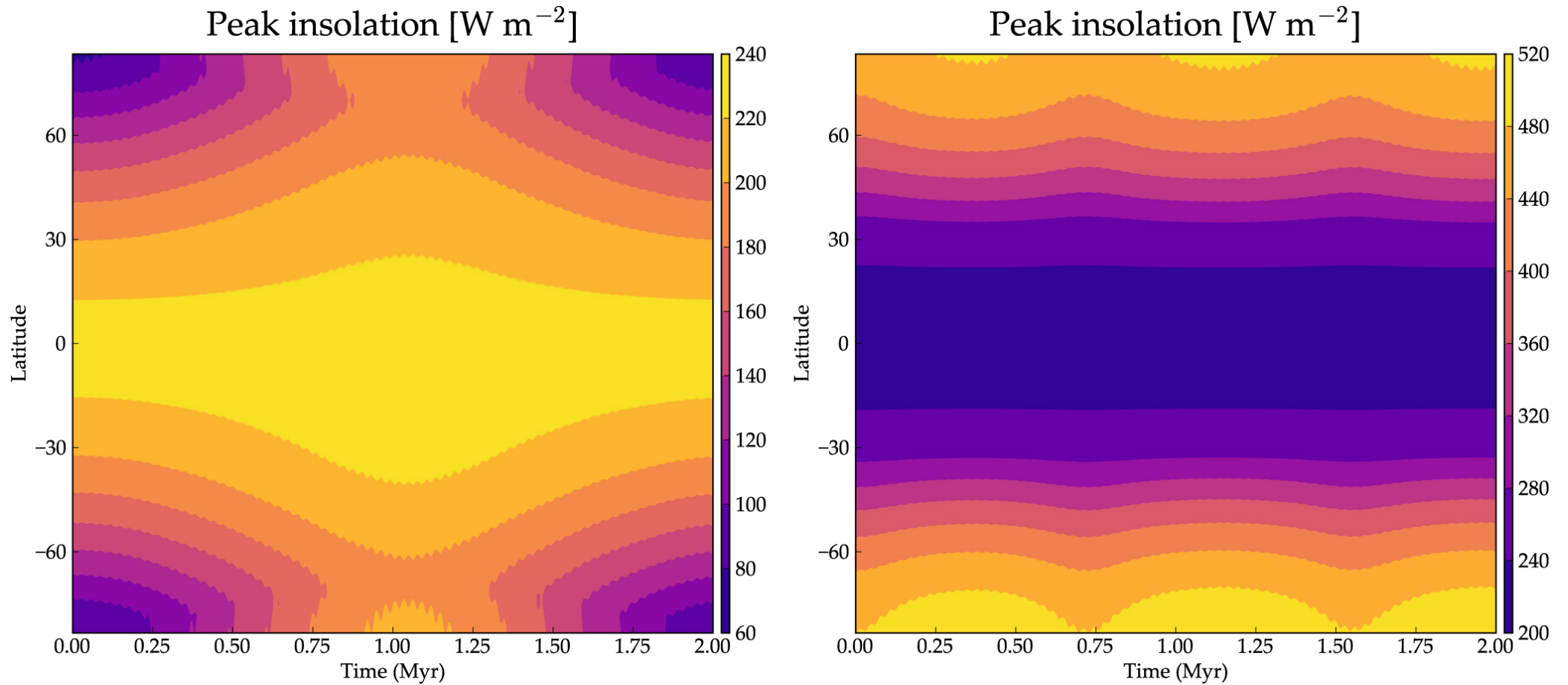
Figure 19. from Exo-Milankovitch Cycles. I. Orbits and Rotation States null 2018 AJ 155 60 doi:10.3847/1538-3881/aaa301 https://dx.doi.org/10.3847/1538-3881/aaa301 © 2018. The American Astronomical Society. All rights reserved.
