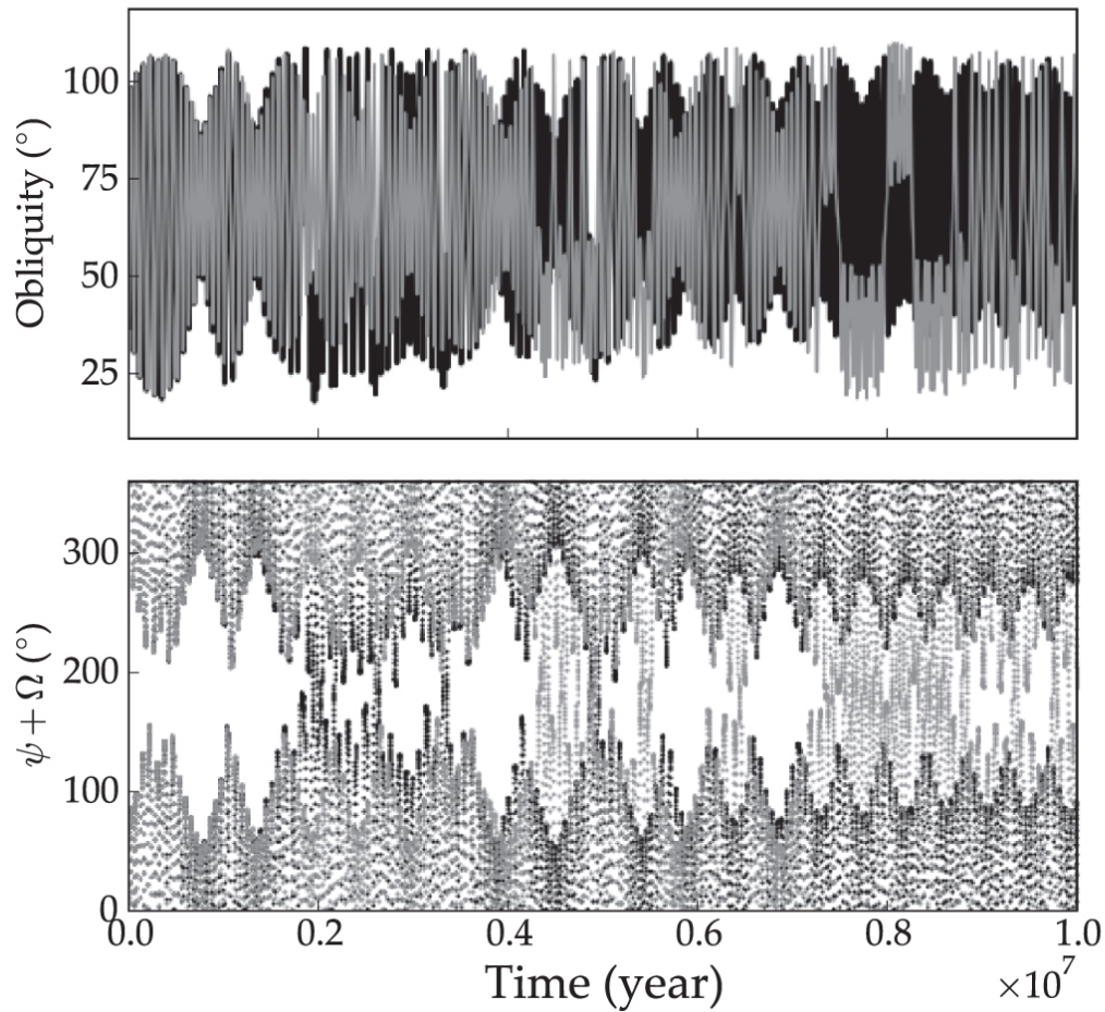
Figure 18. from Exo-Milankovitch Cycles. I. Orbits and Rotation States null 2018 AJ 155 60 doi:10.3847/1538-3881/aaa301 https://dx.doi.org/10.3847/1538-3881/aaa301 © 2018. The American Astronomical Society. All rights reserved.
