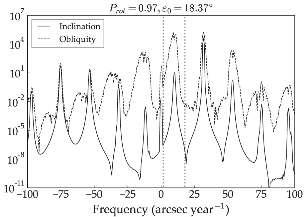
Figure 17. from Exo-Milankovitch Cycles. I. Orbits and Rotation States null 2018 AJ 155 60 doi:10.3847/1538-3881/aaa301 https://dx.doi.org/10.3847/1538-3881/aaa301 © 2018. The American Astronomical Society. All rights reserved.
