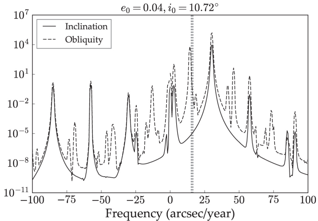
Figure 16. from Exo-Milankovitch Cycles. I. Orbits and Rotation States null 2018 AJ 155 60 doi:10.3847/1538-3881/aaa301 https://dx.doi.org/10.3847/1538-3881/aaa301 © 2018. The American Astronomical Society. All rights reserved.
