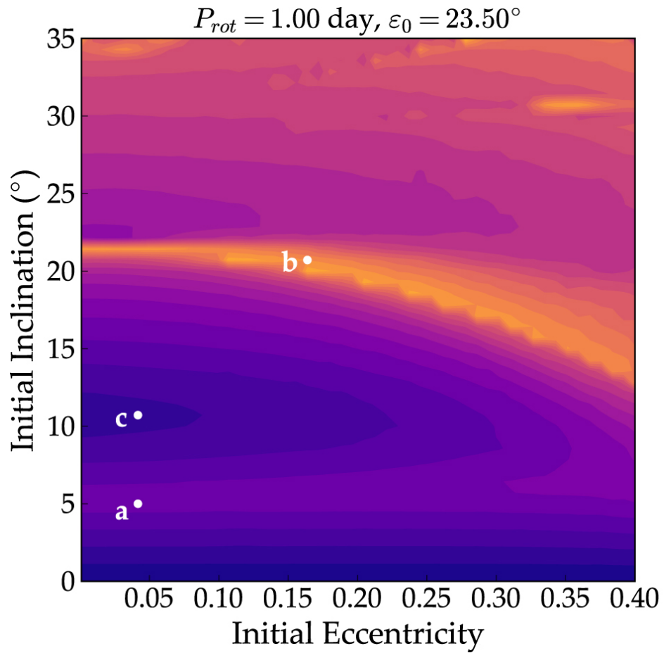
Figure 13. from Exo-Milankovitch Cycles. I. Orbits and Rotation States null 2018 AJ 155 60 doi:10.3847/1538-3881/aaa301 https://dx.doi.org/10.3847/1538-3881/aaa301 © 2018. The American Astronomical Society. All rights reserved.
