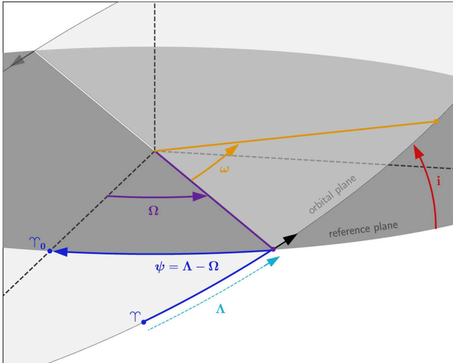
Figure 1. from Exo-Milankovitch Cycles. I. Orbits and Rotation States null 2018 AJ 155 60 doi:10.3847/1538-3881/aaa301 https://dx.doi.org/10.3847/1538-3881/aaa301 © 2018. The American Astronomical Society. All rights reserved.
