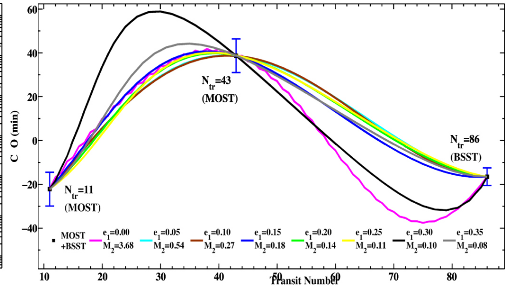
Figure 7. from Searching for the Transit of the Earth-mass Exoplanet Proxima Centauri b in Antarctica: Preliminary Result null 2018 AJ 155 12 doi:10.3847/1538-3881/aa9b86 https://dx.doi.org/10.3847/1538-3881/aa9b86 © 2017. The American Astronomical Society. All rights reserved.
