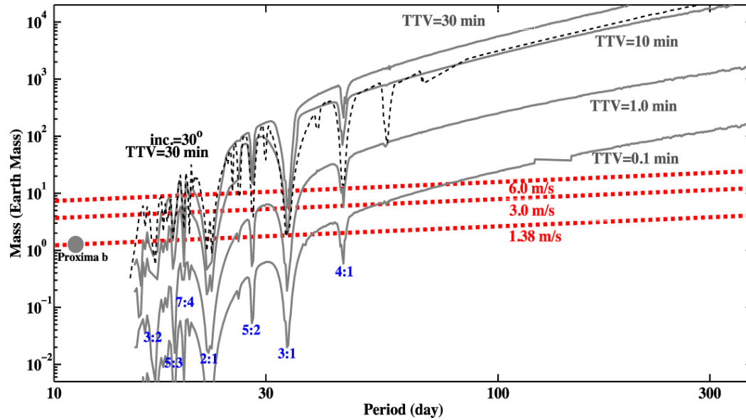
Figure 7. from Searching for the Transit of the Earth-mass Exoplanet Proxima Centauri b in Antarctica: Preliminary Result null 2018 AJ 155 12 doi:10.3847/1538-3881/aa9b86 https://dx.doi.org/10.3847/1538-3881/aa9b86 © 2017. The American Astronomical Society. All rights reserved.
