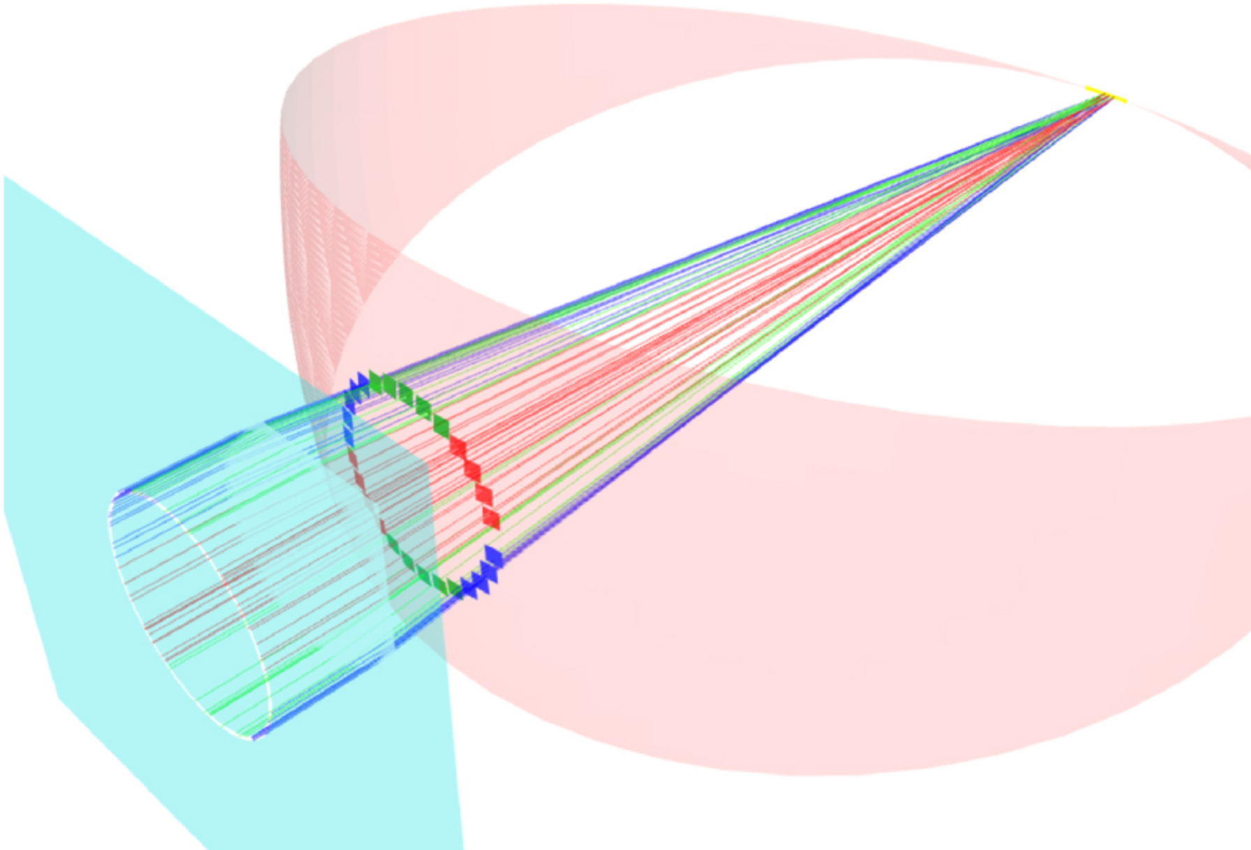
Figure 1. from MARXS: A Modular Software to Ray-trace X-Ray Instrumentation null 2017 AJ 154 243 doi:10.3847/1538-3881/aa943b https://dx.doi.org/10.3847/1538-3881/aa943b © 2017. The American Astronomical Society. All rights reserved.
