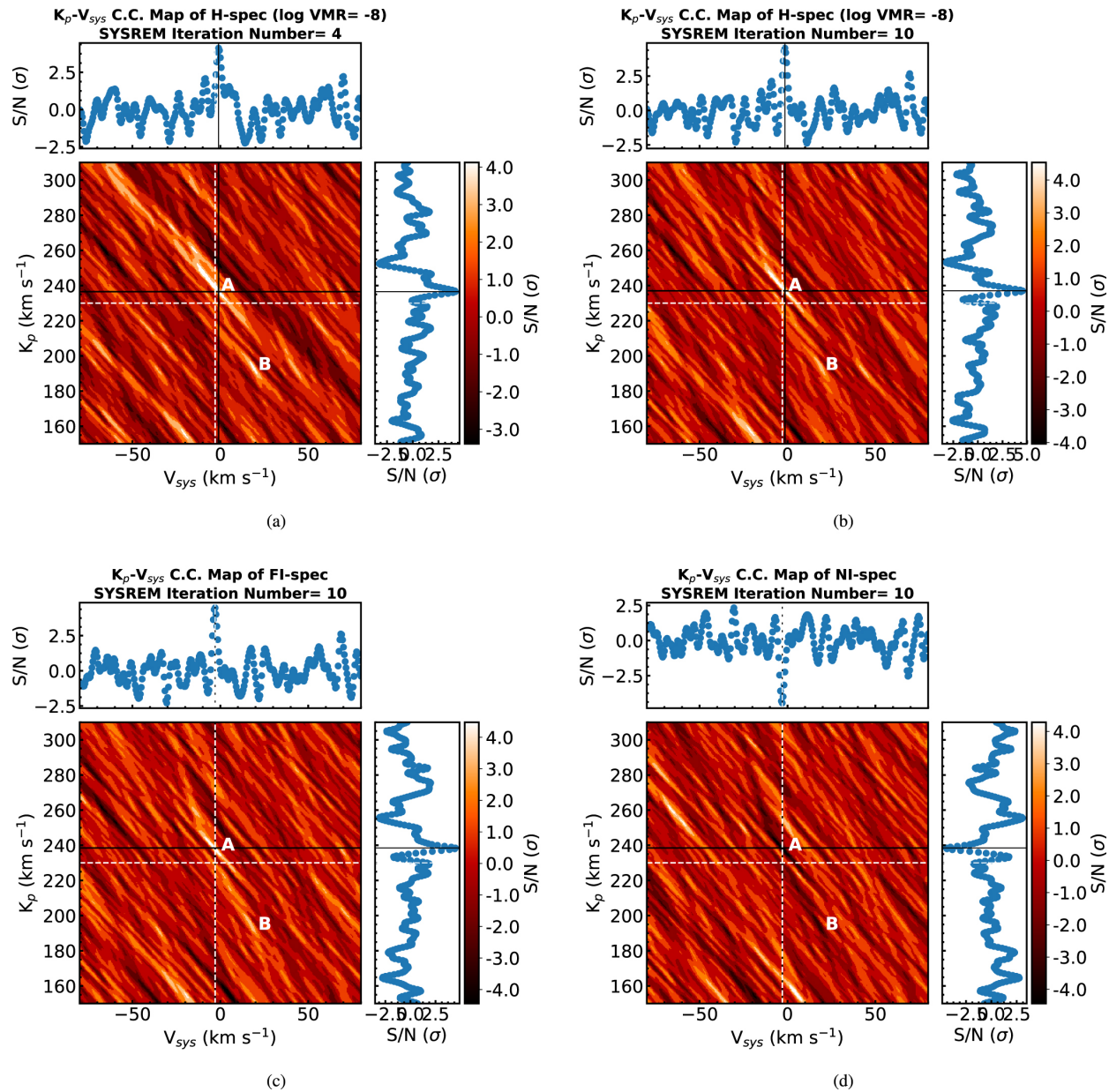
Figure 9. from High-resolution Spectroscopic Detection of TiO and a Stratosphere in the Day-side of WASP-33b null 2017 AJ 154 221 doi:10.3847/1538-3881/aa9433 https://dx.doi.org/10.3847/1538-3881/aa9433
