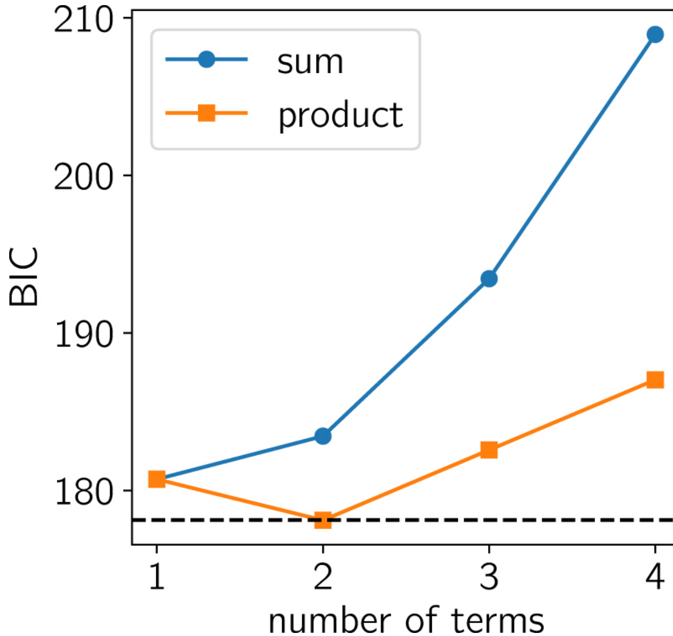
Figure 6. from Fast and Scalable Gaussian Process Modeling with Applications to Astronomical Time Series null 2017 AJ 154 220 doi:10.3847/1538-3881/aa9332 https://dx.doi.org/10.3847/1538-3881/aa9332 © 2017. The American Astronomical Society. All rights reserved.
