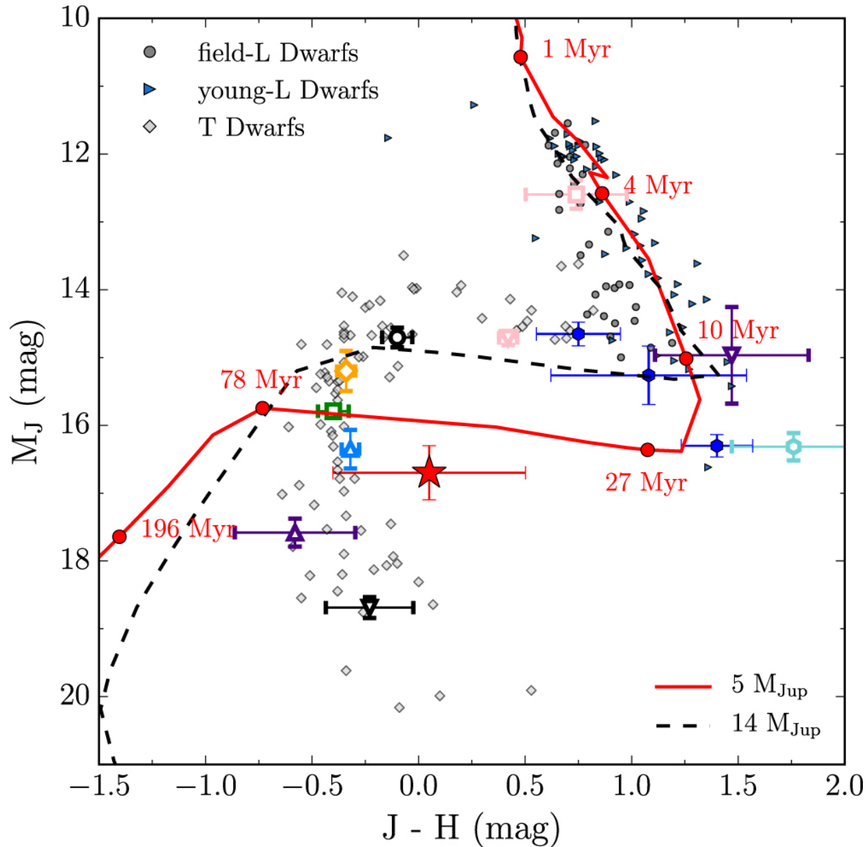
Figure 9. from Characterizing 51 Eri b from 1 to 5 m: A Partly Cloudy Exoplanet null 2017 AJ 154 10 doi:10.3847/1538-3881/aa74db https://dx.doi.org/10.3847/1538-3881/aa74db © 2017. The American Astronomical Society. All rights reserved.
