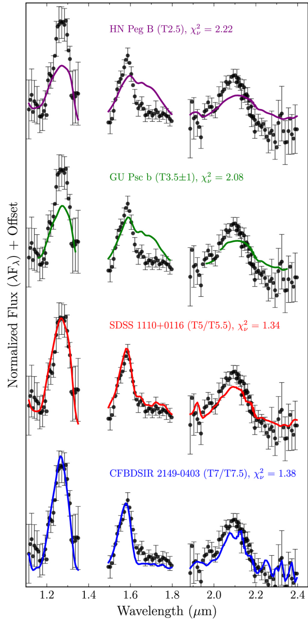
Figure 8. from Characterizing 51 Eri b from 1 to 5 m: A Partly Cloudy Exoplanet null 2017 AJ 154 10 doi:10.3847/1538-3881/aa74db https://dx.doi.org/10.3847/1538-3881/aa74db © 2017. The American Astronomical Society. All rights reserved.
