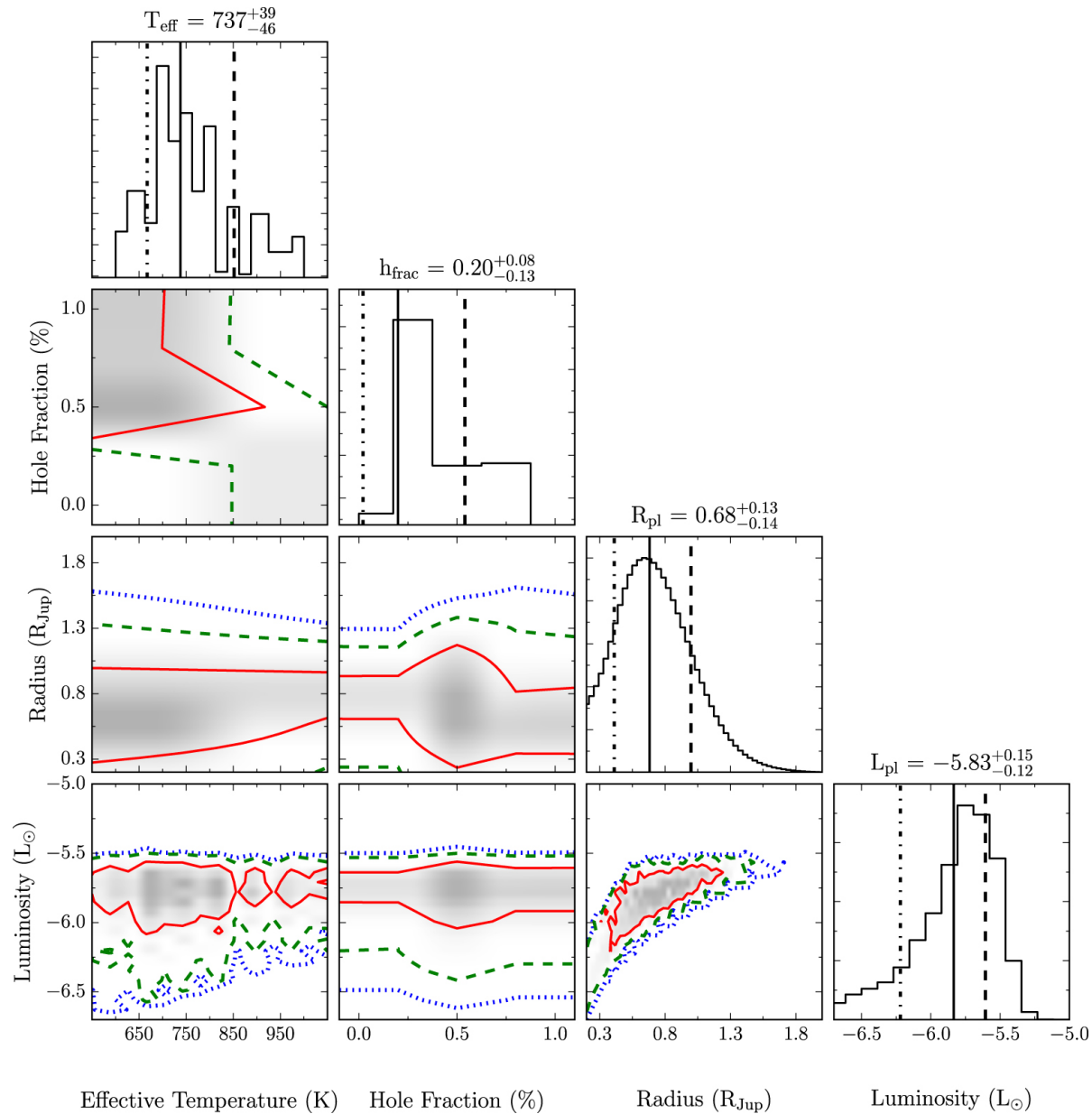
Figure 11. from Characterizing 51 Eri b from 1 to 5 m: A Partly Cloudy Exoplanet null 2017 AJ 154 10 doi:10.3847/1538-3881/aa74db https://dx.doi.org/10.3847/1538-3881/aa74db © 2017. The American Astronomical Society. All rights reserved.
