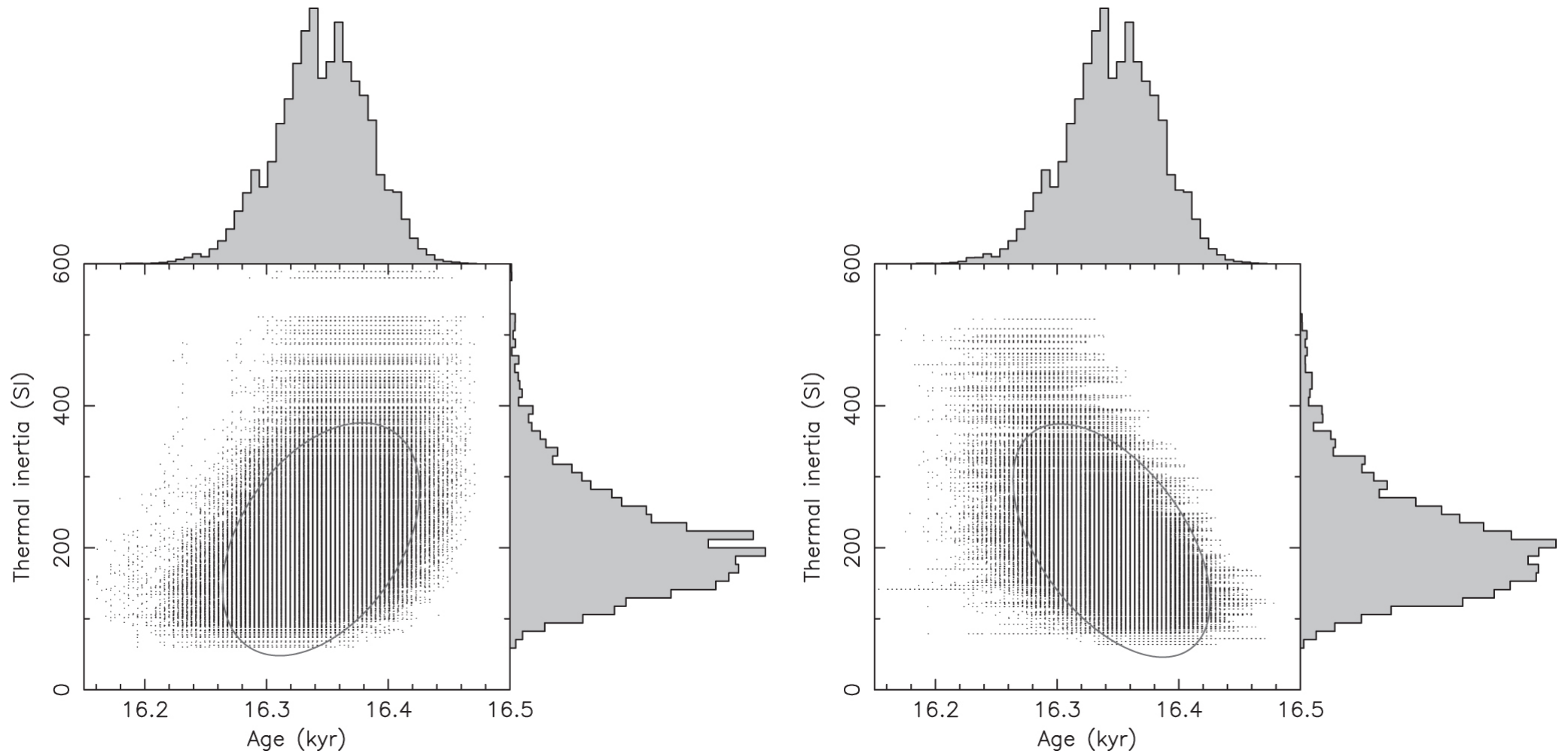
Figure 9. from Detailed Analysis of the Asteroid Pair (6070) Rheinland and (54827) 2001 NQ8 null 2017 AJ 153 270 doi:10.3847/1538-3881/aa72ea https://dx.doi.org/10.3847/1538-3881/aa72ea © 2017. The American Astronomical Society. All rights reserved.
