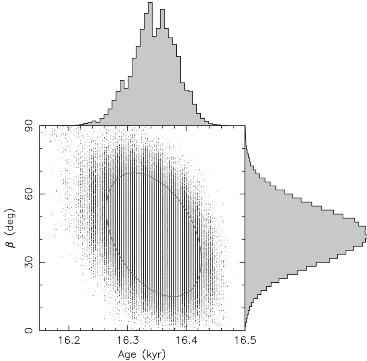
Figure 8. from Detailed Analysis of the Asteroid Pair (6070) Rheinland and (54827) 2001 NQ8 null 2017 AJ 153 270 doi:10.3847/1538-3881/aa72ea https://dx.doi.org/10.3847/1538-3881/aa72ea © 2017. The American Astronomical Society. All rights reserved.
