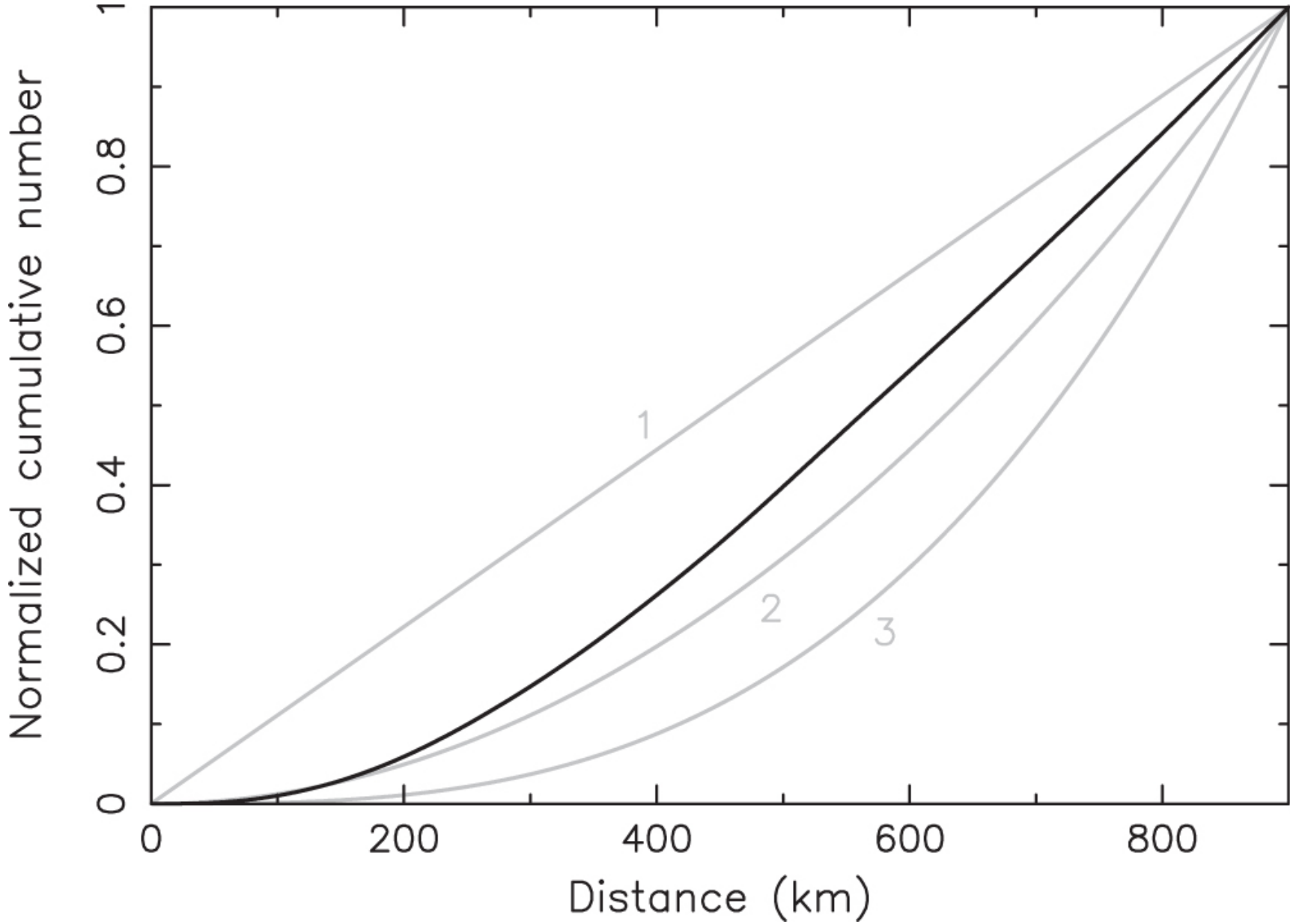
Figure 7. from Detailed Analysis of the Asteroid Pair (6070) Rheinland and (54827) 2001 NQ8 null 2017 AJ 153 270 doi:10.3847/1538-3881/aa72ea https://dx.doi.org/10.3847/1538-3881/aa72ea © 2017. The American Astronomical Society. All rights reserved.
