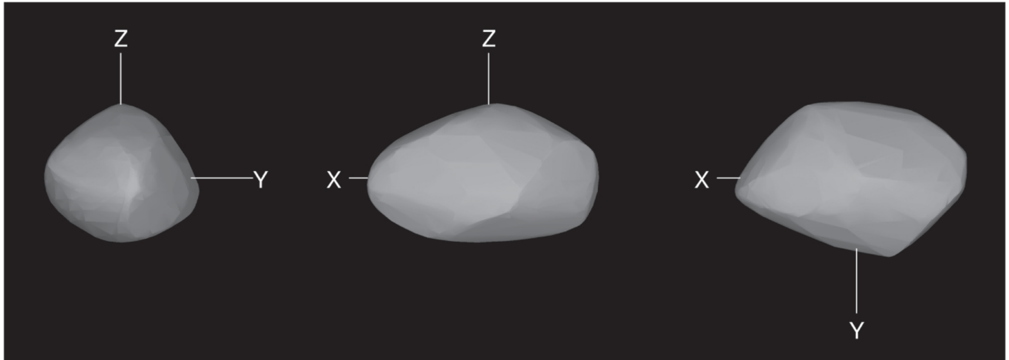
Figure 4. from Detailed Analysis of the Asteroid Pair (6070) Rheinland and (54827) 2001 NQ8 null 2017 AJ 153 270 doi:10.3847/1538-3881/aa72ea https://dx.doi.org/10.3847/1538-3881/aa72ea © 2017. The American Astronomical Society. All rights reserved.
