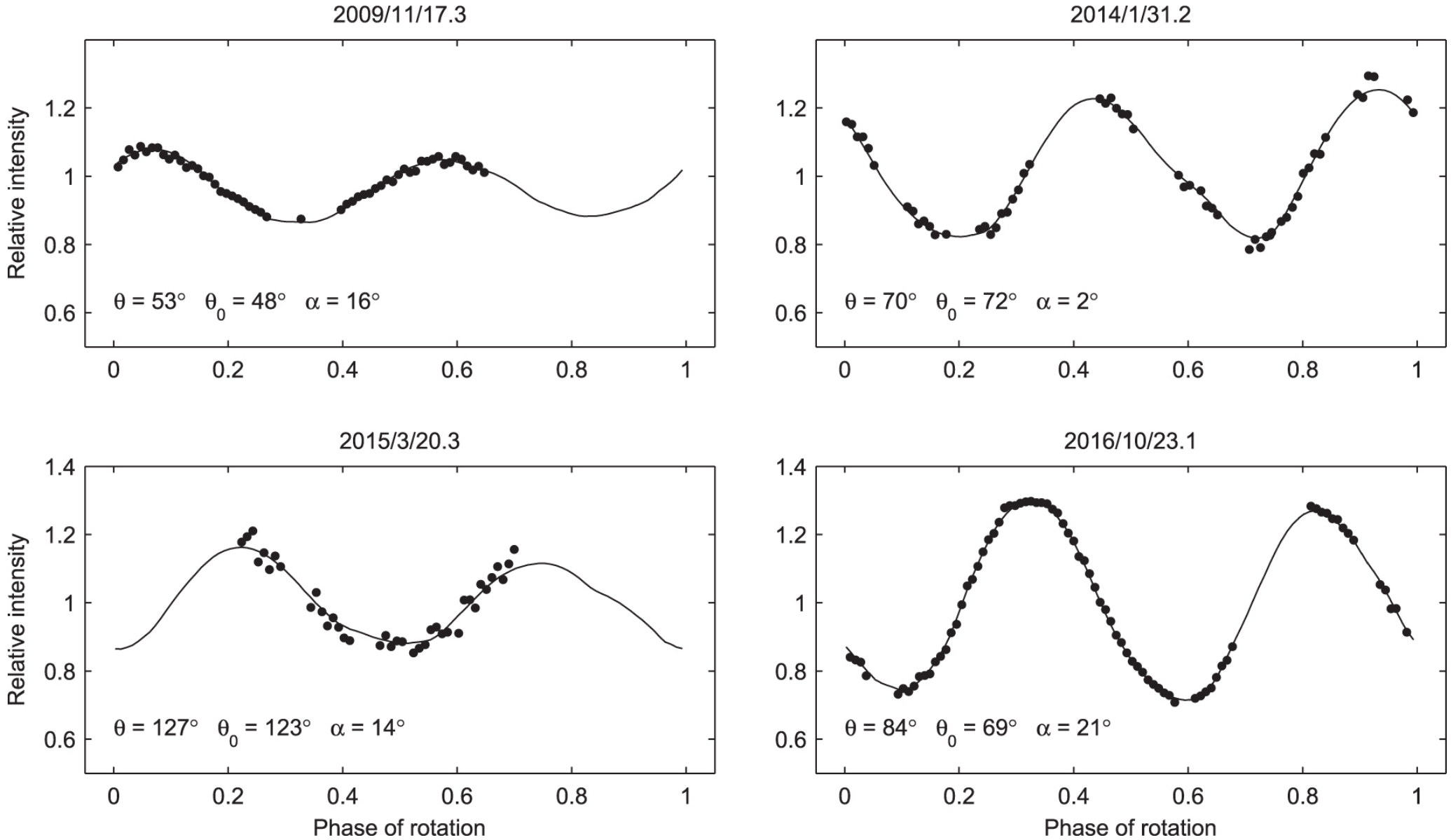
Figure 3. from Detailed Analysis of the Asteroid Pair (6070) Rheinland and (54827) 2001 NQ8 null 2017 AJ 153 270 doi:10.3847/1538-3881/aa72ea https://dx.doi.org/10.3847/1538-3881/aa72ea © 2017. The American Astronomical Society. All rights reserved.
