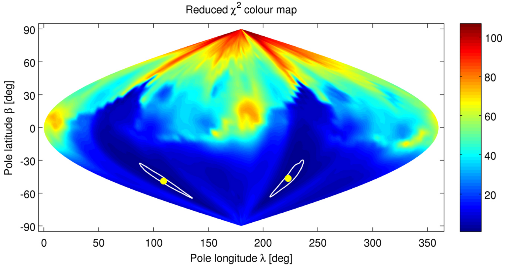
Figure 2. from Detailed Analysis of the Asteroid Pair (6070) Rheinland and (54827) 2001 NQ8 null 2017 AJ 153 270 doi:10.3847/1538-3881/aa72ea https://dx.doi.org/10.3847/1538-3881/aa72ea © 2017. The American Astronomical Society. All rights reserved.
