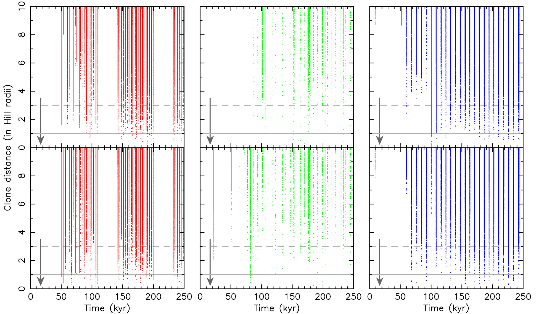
Figure 12. from Detailed Analysis of the Asteroid Pair (6070) Rheinland and (54827) 2001 NQ8 null 2017 AJ 153 270 doi:10.3847/1538-3881/aa72ea https://dx.doi.org/10.3847/1538-3881/aa72ea © 2017. The American Astronomical Society. All rights reserved.
