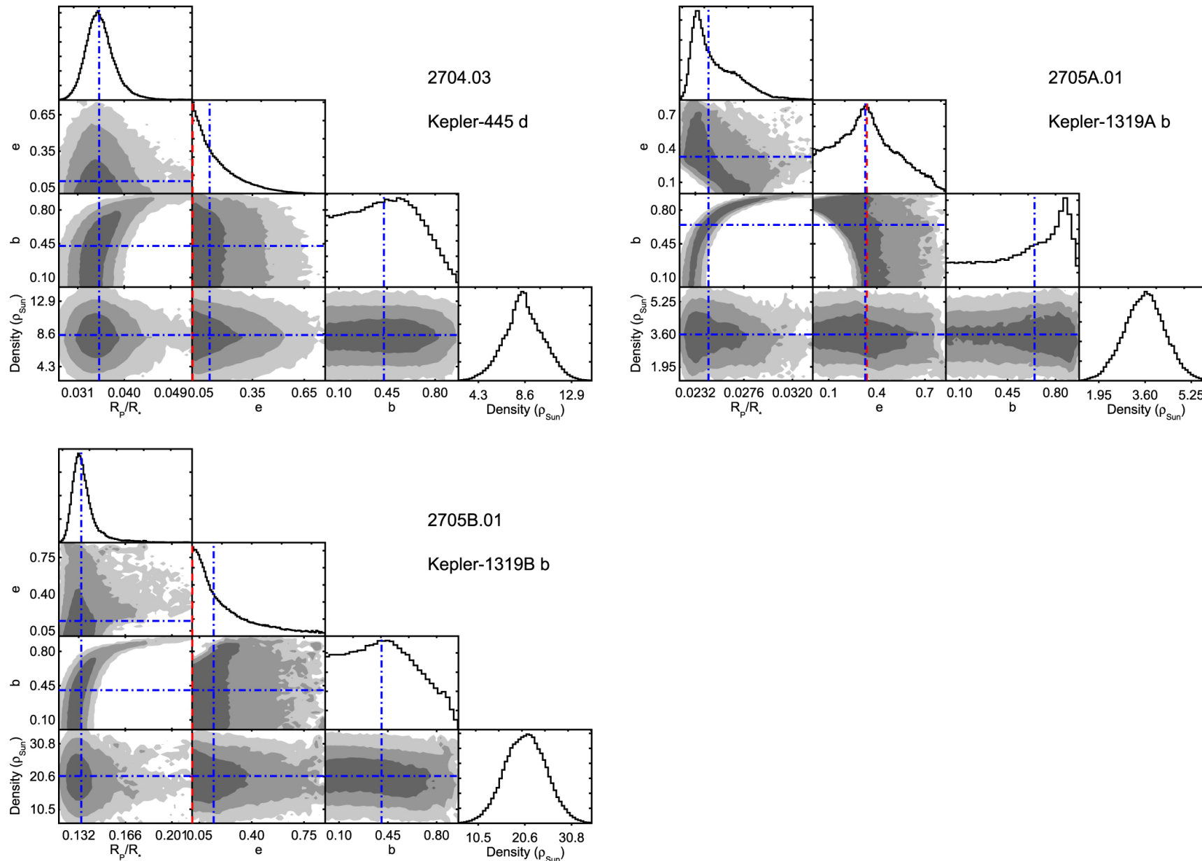
Figure 10. from The Gold Standard: Accurate Stellar and Planetary Parameters for Eight Kepler M Dwarf Systems Enabled by Parallaxes null 2017 AJ 153 267 doi:10.3847/1538-3881/aa7140 https://dx.doi.org/10.3847/1538-3881/aa7140 © 2017. The American Astronomical Society. All rights reserved.
