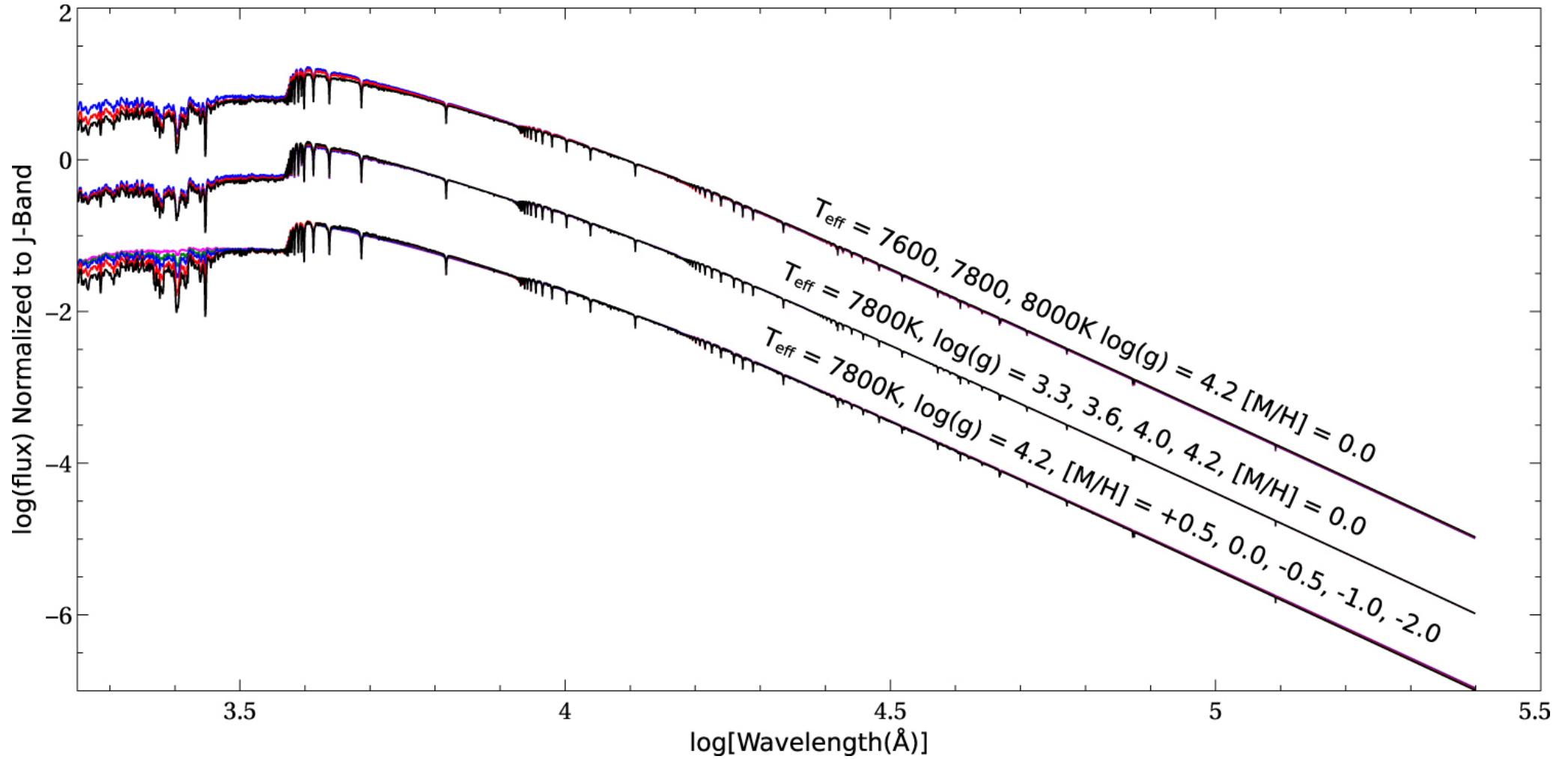
Figure 2. from The Discovery of Bootis Stars: The Southern Survey I null 2017 AJ 154 31 doi:10.3847/1538-3881/aa6d5e https://dx.doi.org/10.3847/1538-3881/aa6d5e © 2017. The American Astronomical Society. All rights reserved.
